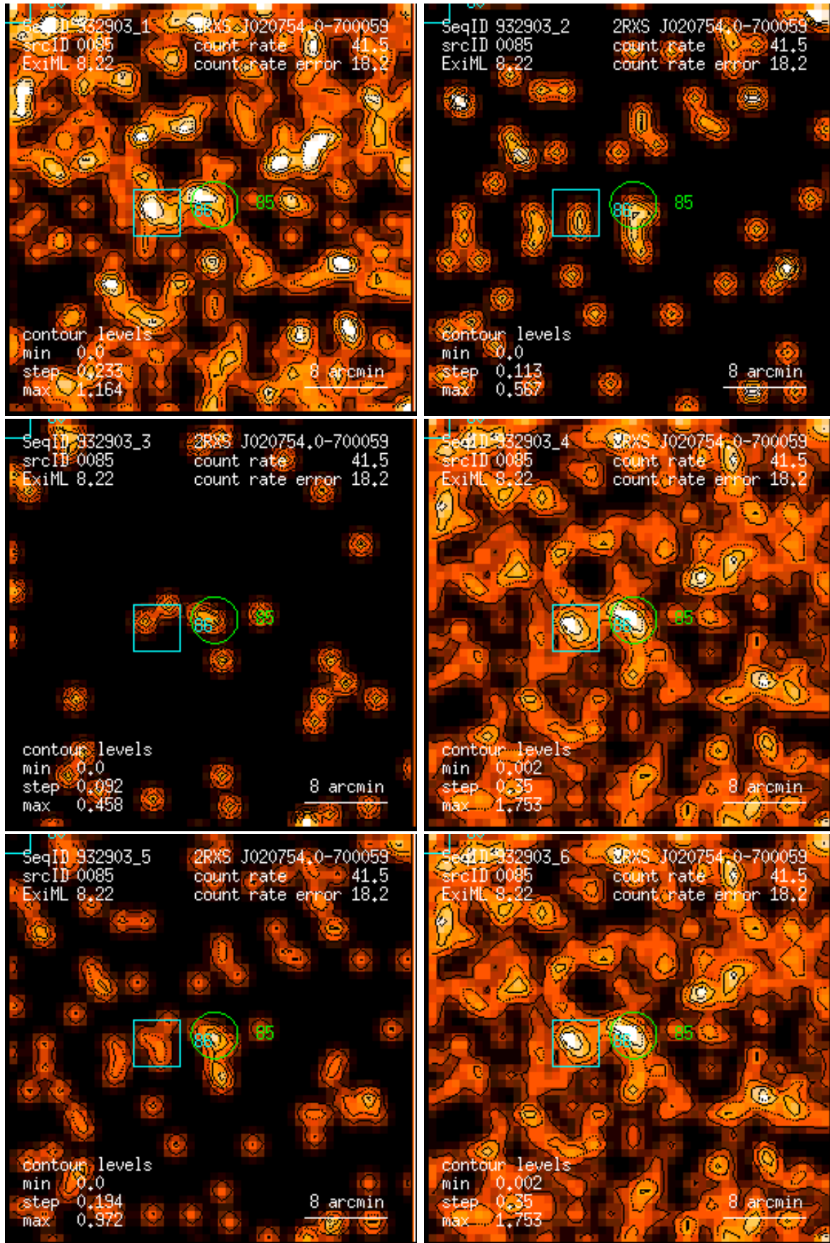
Figure 85: RASS 932903: detection 0085: band rate images, Gaussian filter: (1) PSPC channels 11 – 41, (2) 52 – 90, (3) 91 – 201, (4) 11 – 235, (5) 52 – 201, (6) 11 – 201. Broad band rates in counts/ks. Band rate contour levels in counts/ks/arcmin 2 .
