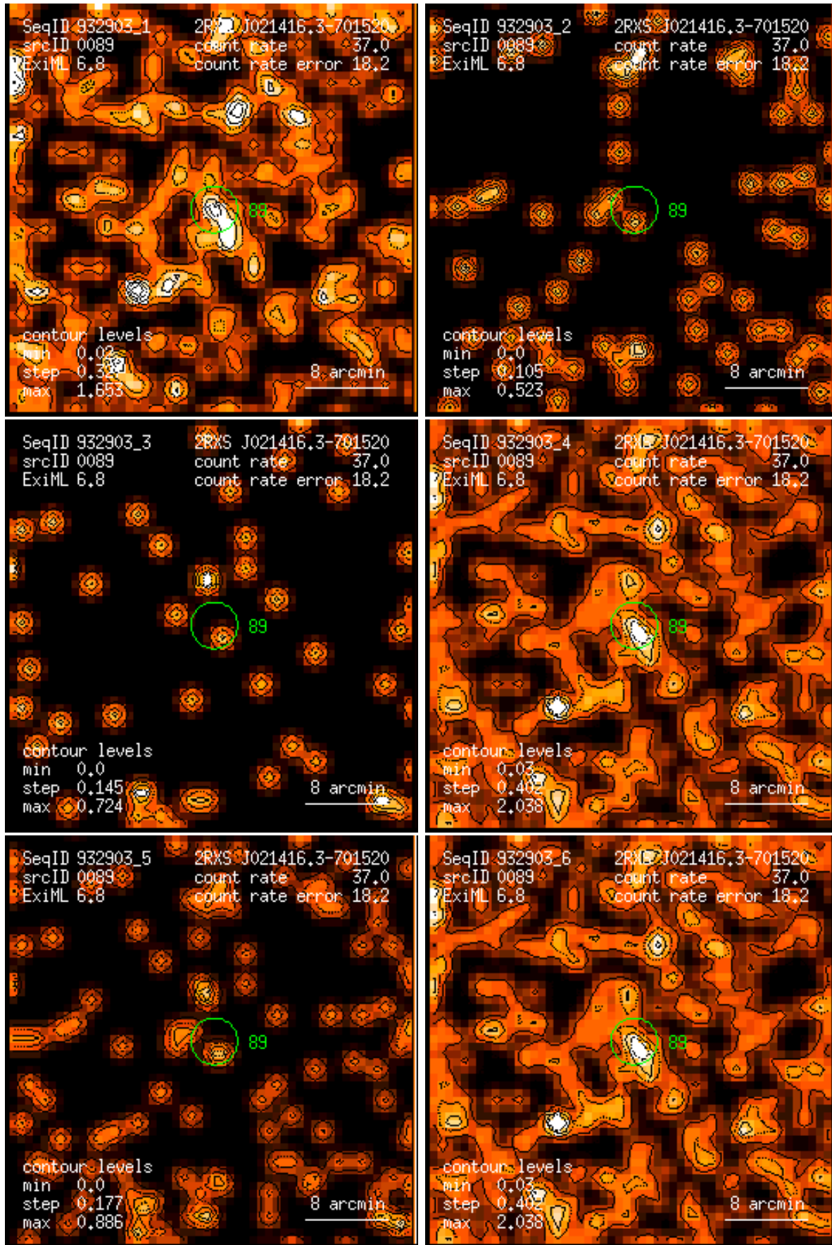
Figure 89: RASS 932903: detection 0089: band rate images, Gaussian filter: (1) PSPC channels 11 – 41, (2) 52 – 90, (3) 91 – 201, (4) 11 – 235, (5) 52 – 201, (6) 11 – 201. Broad band rates in counts/ks. Band rate contour levels in counts/ks/arcmin 2 .
