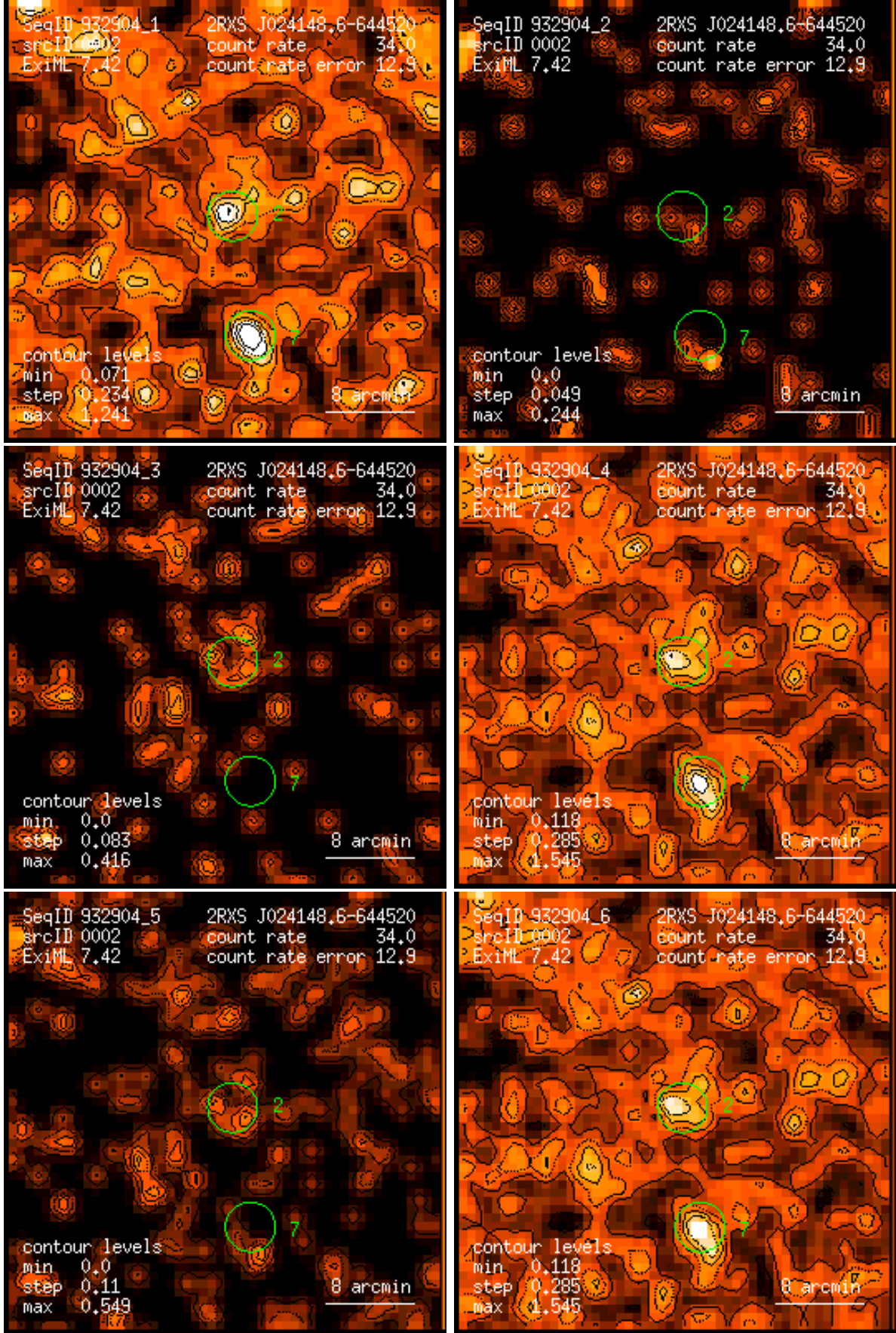
Figure 2: RASS 932904: detection 0002: band rate images, Gaussian filter: (1) PSPC channels 11 – 41, (2) 52 – 90, (3) 91 – 201, (4) 11 – 235, (5) 52 – 201, (6) 11 – 201. Broad band rates in counts/ks. Band rate contour levels in counts/ks/arcmin 2 .
