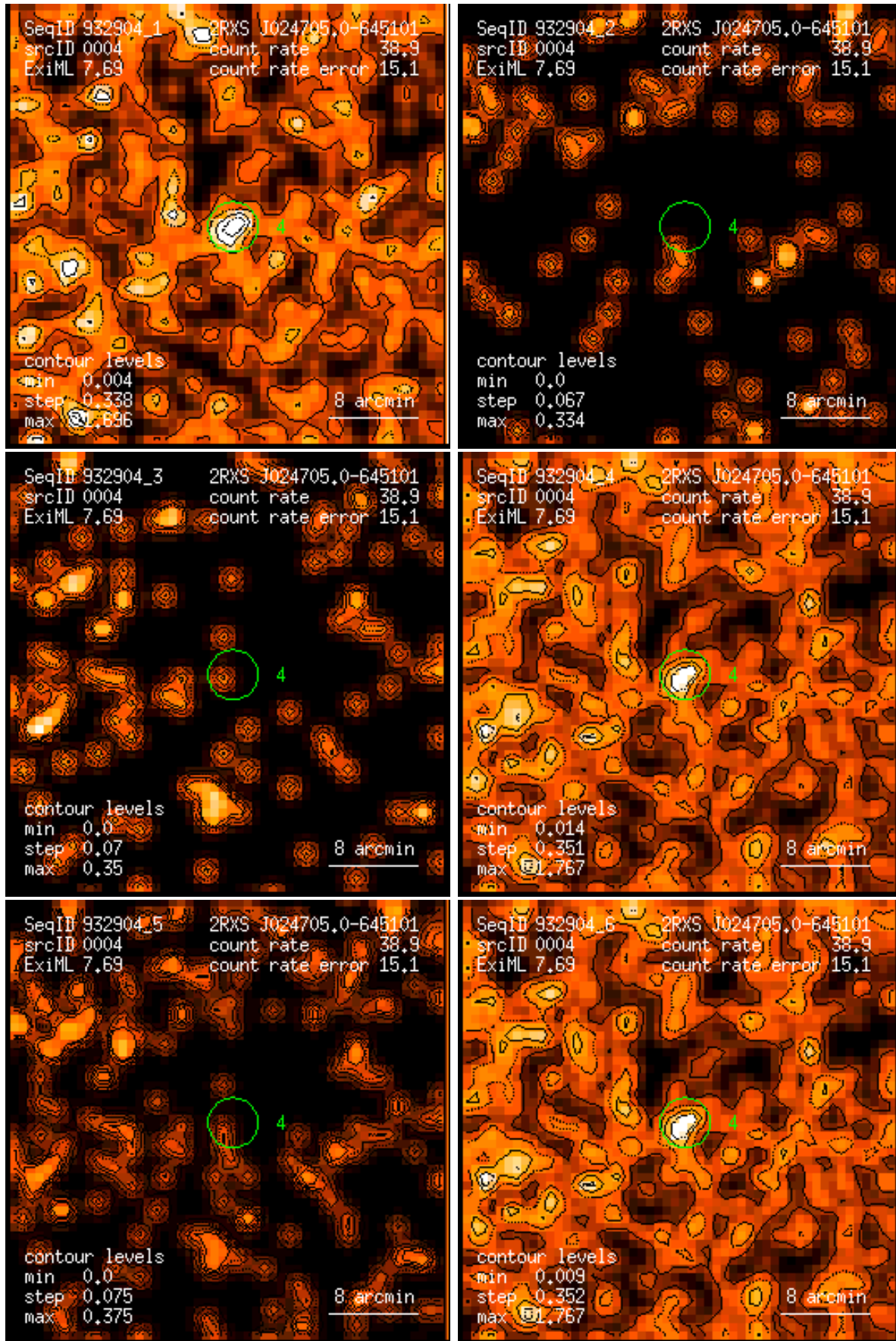
Figure 4: RASS 932904: detection 0004: band rate images, Gaussian filter: (1) PSPC channels 11 – 41, (2) 52 – 90, (3) 91 – 201, (4) 11 – 235, (5) 52 – 201, (6) 11 – 201. Broad band rates in counts/ks. Band rate contour levels in counts/ks/arcmin 2 .
