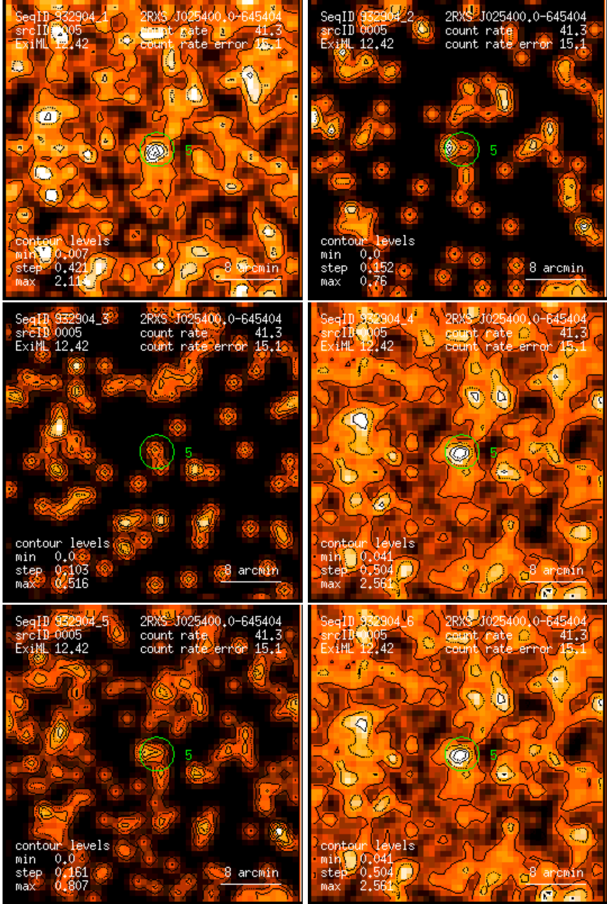
Figure 5: RASS 932904: detection 0005: band rate images, Gaussian filter: (1) PSPC channels 11 – 41, (2) 52 – 90, (3) 91 – 201, (4) 11 – 235, (5) 52 – 201, (6) 11 – 201. Broad band rates in counts/ks. Band rate contour levels in counts/ks/arcmin 2 .
