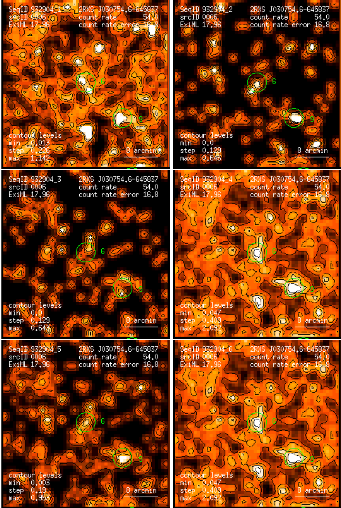
Figure 6: RASS 932904: detection 0006: band rate images, Gaussian filter: (1) PSPC channels 11 – 41, (2) 52 – 90, (3) 91 – 201, (4) 11 – 235, (5) 52 – 201, (6) 11 – 201. Broad band rates in counts/ks. Band rate contour levels in counts/ks/arcmin 2 .
