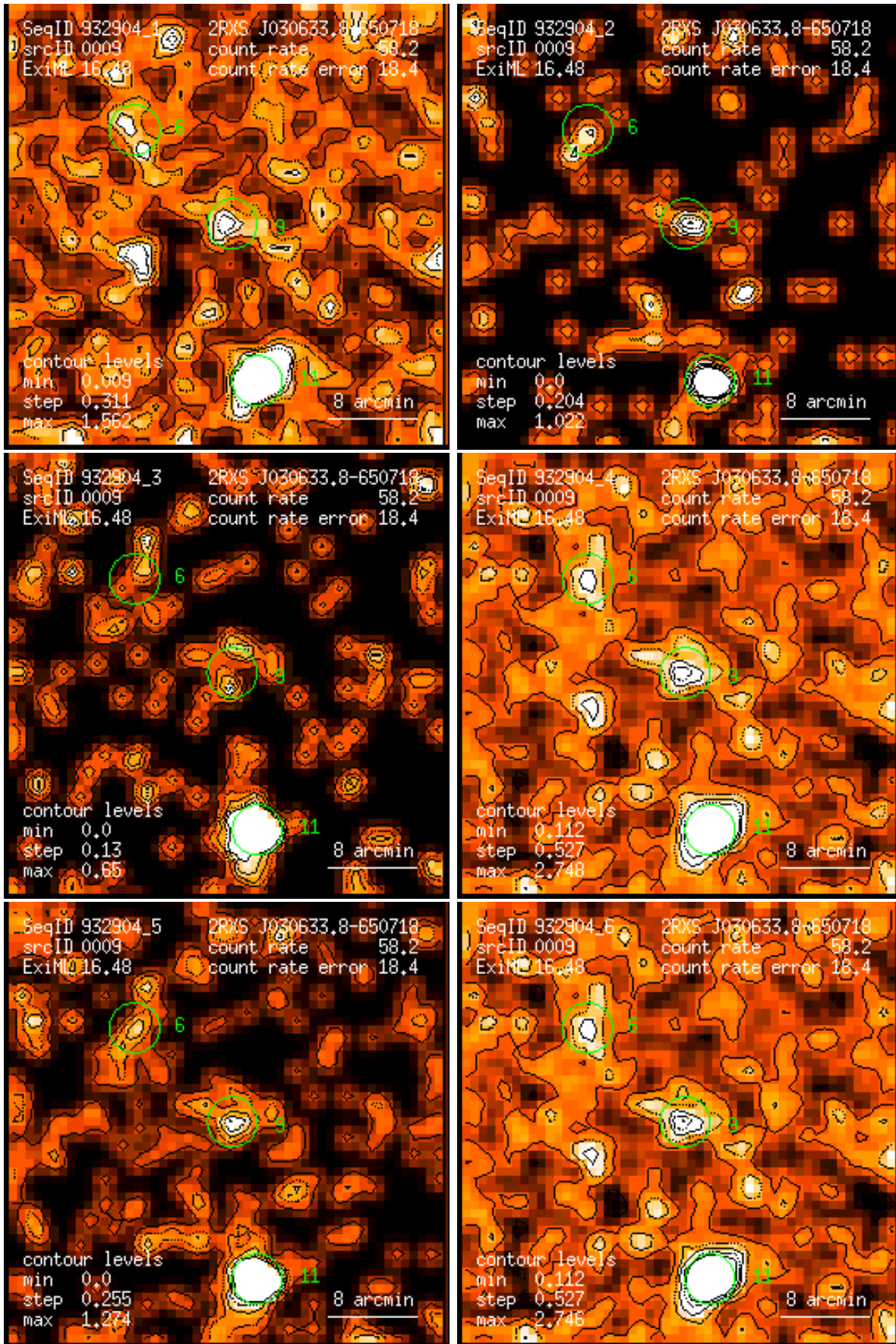
Figure 9: RASS 932904: detection 0009: band rate images, Gaussian filter: (1) PSPC channels 11 – 41, (2) 52 – 90, (3) 91 – 201, (4) 11 – 235, (5) 52 – 201, (6) 11 – 201. Broad band rates in counts/ks. Band rate contour levels in counts/ks/arcmin 2 .
