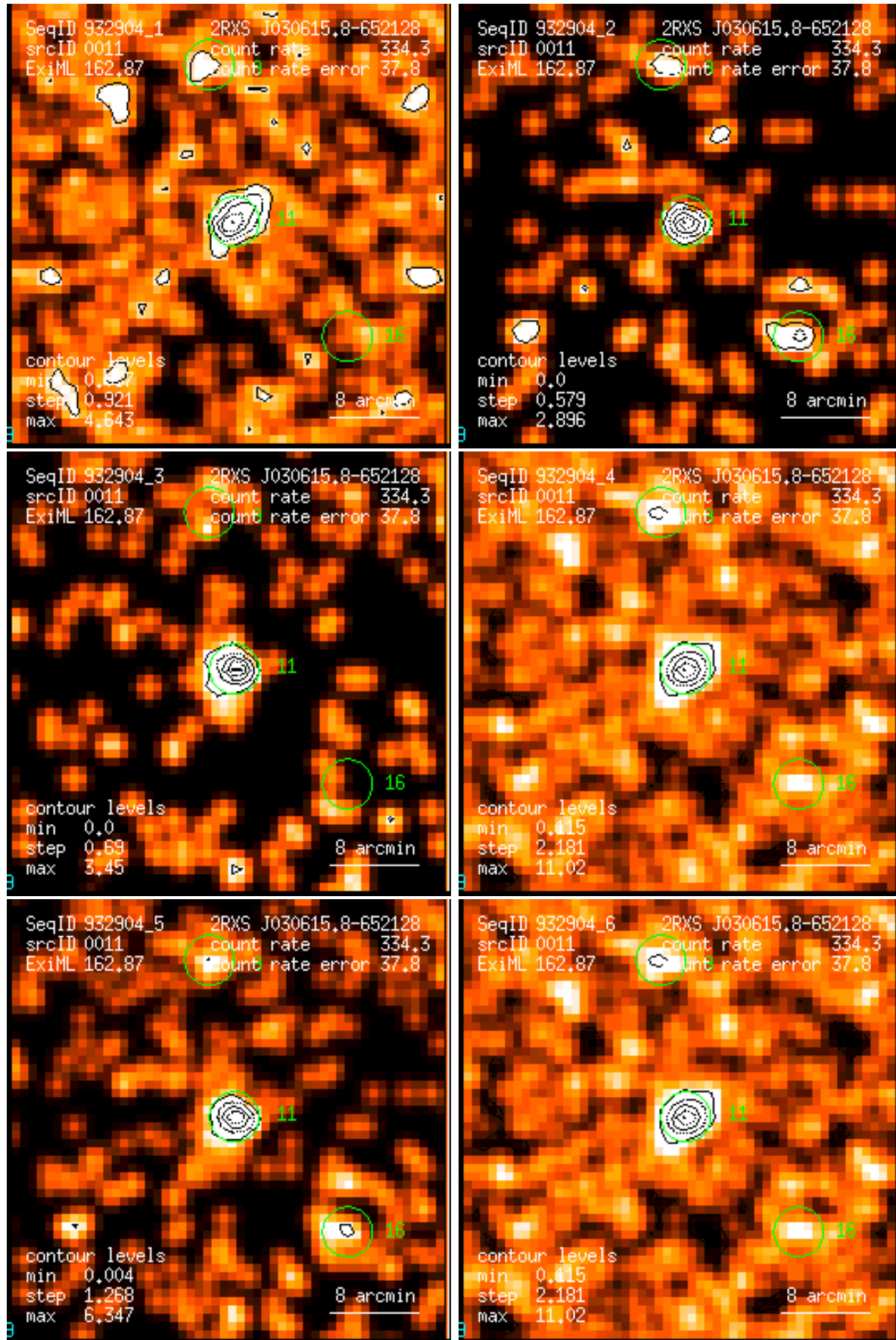
Figure 11: RASS 932904: detection 0011: band rate images, Gaussian filter: (1) PSPC channels 11 – 41, (2) 52 – 90, (3) 91 – 201, (4) 11 – 235, (5) 52 – 201, (6) 11 – 201. Broad band rates in counts/ks. Band rate contour levels in counts/ks/arcmin 2 .
