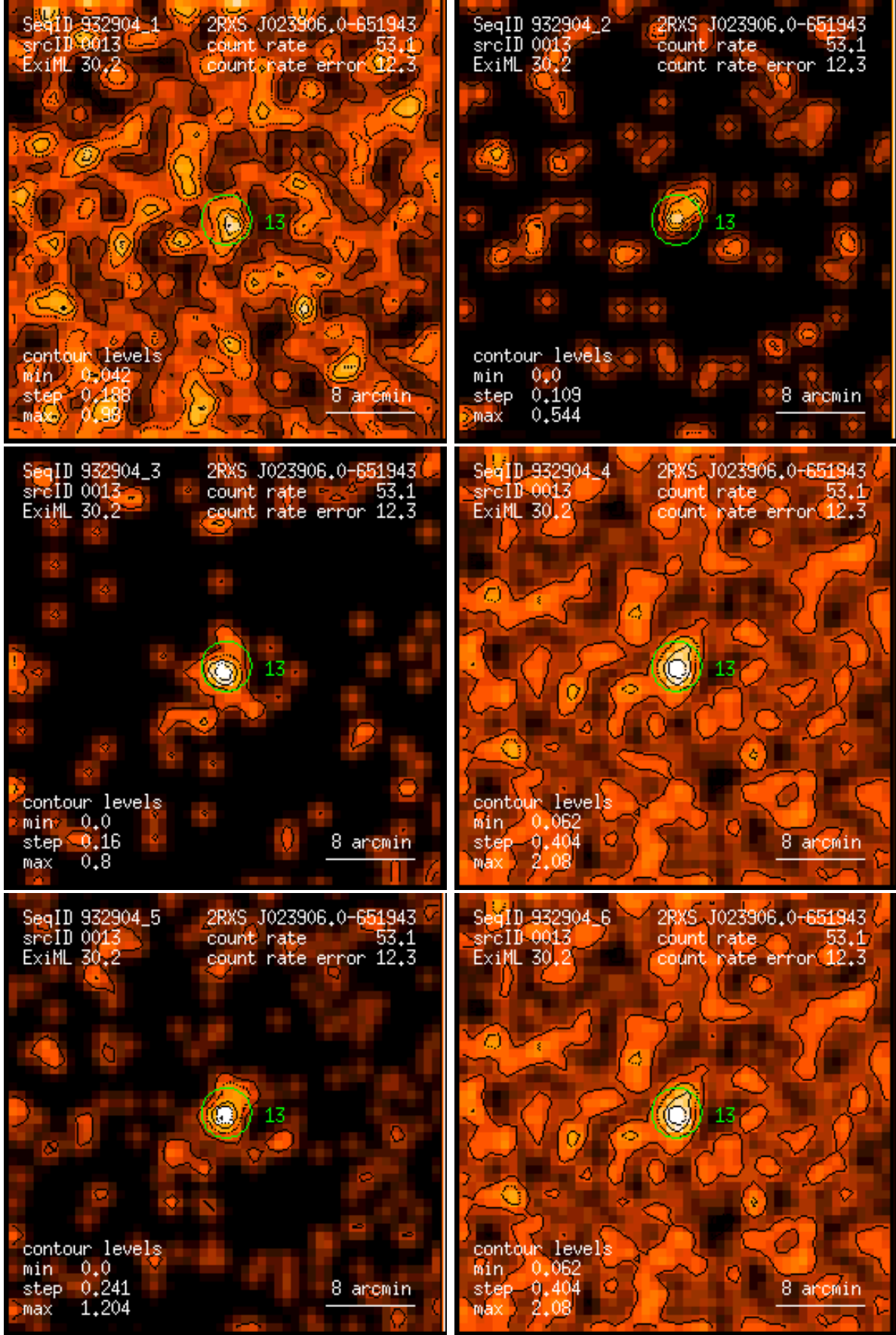
Figure 13: RASS 932904: detection 0013: band rate images, Gaussian filter: (1) PSPC channels 11 – 41, (2) 52 – 90, (3) 91 – 201, (4) 11 – 235, (5) 52 – 201, (6) 11 – 201. Broad band rates in counts/ks. Band rate contour levels in counts/ks/arcmin 2 .
