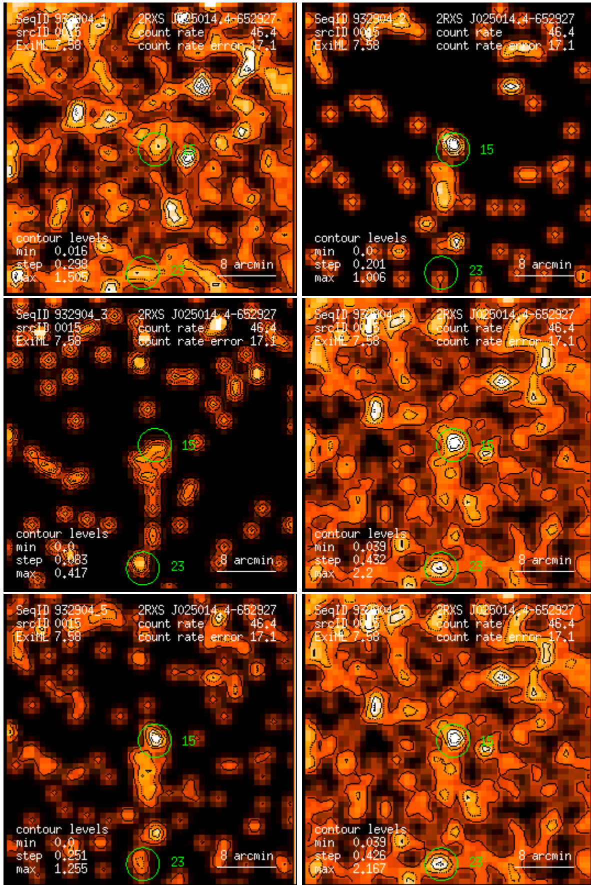
Figure 15: RASS 932904: detection 0015: band rate images, Gaussian filter: (1) PSPC channels 11 – 41, (2) 52 – 90, (3) 91 – 201, (4) 11 – 235, (5) 52 – 201, (6) 11 – 201. Broad band rates in counts/ks. Band rate contour levels in counts/ks/arcmin 2 .
