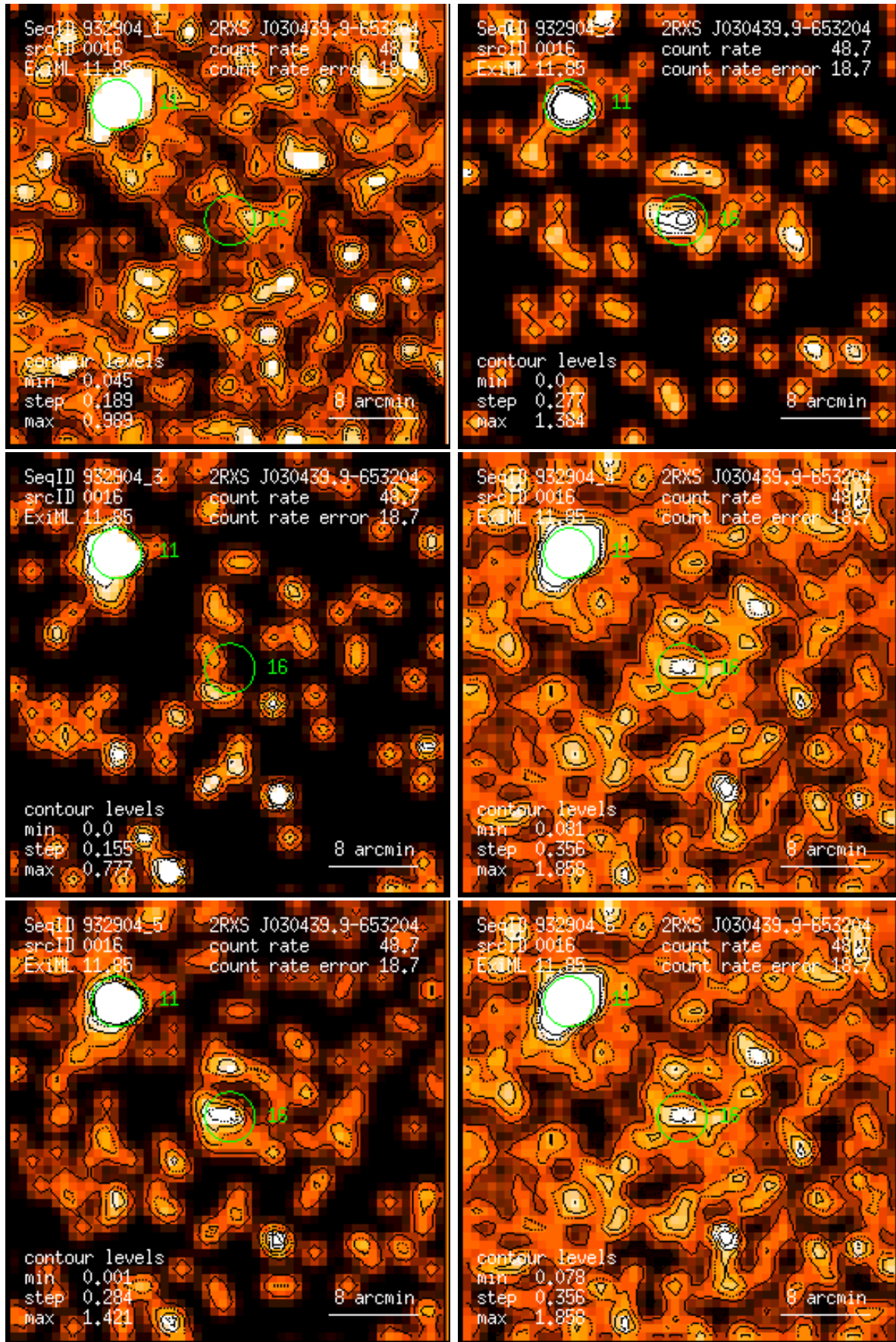
Figure 16: RASS 932904: detection 0016: band rate images, Gaussian filter: (1) PSPC channels 11 – 41, (2) 52 – 90, (3) 91 – 201, (4) 11 – 235, (5) 52 – 201, (6) 11 – 201. Broad band rates in counts/ks. Band rate contour levels in counts/ks/arcmin 2 .
