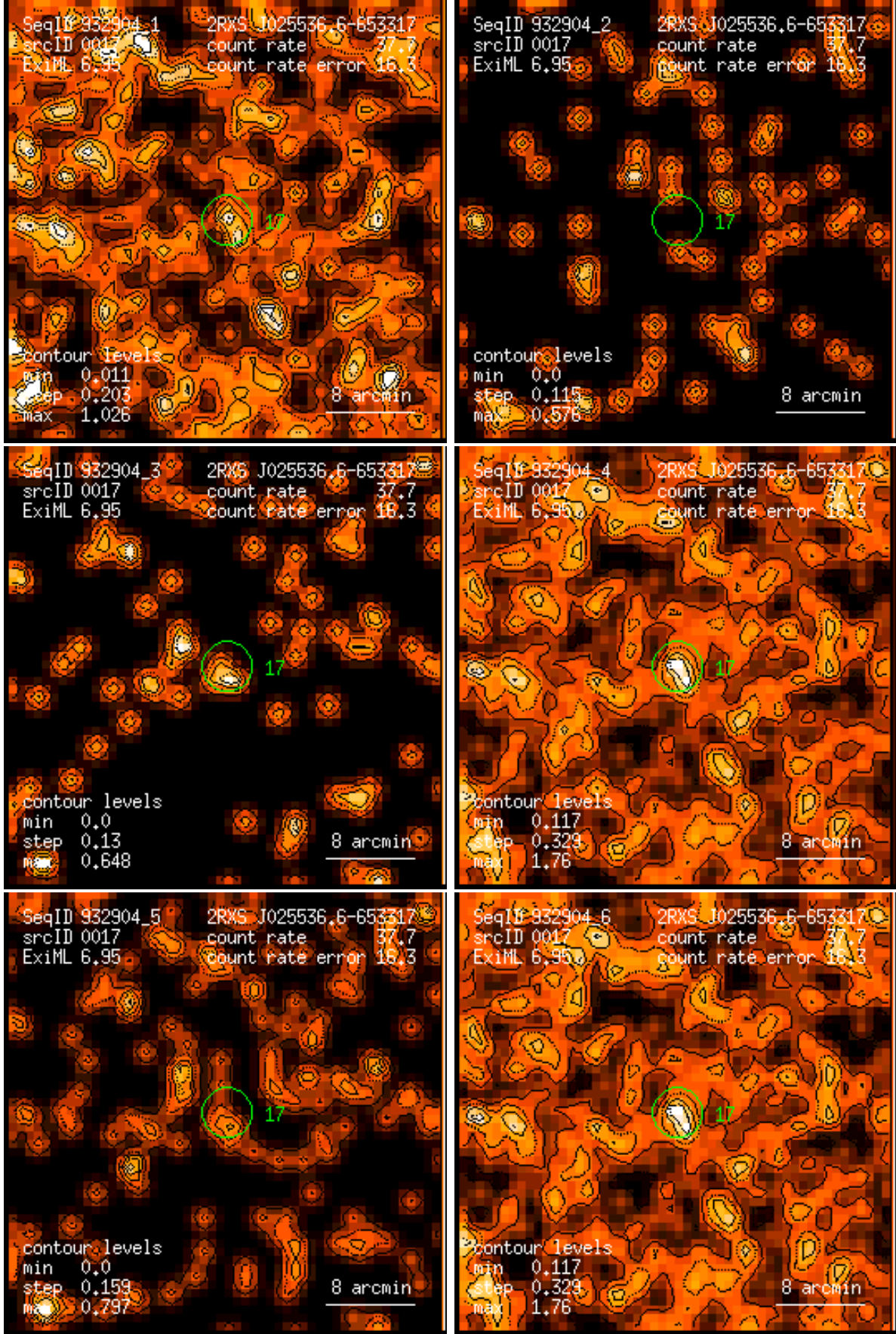
Figure 17: RASS 932904: detection 0017: band rate images, Gaussian filter: (1) PSPC channels 11 – 41, (2) 52 – 90, (3) 91 – 201, (4) 11 – 235, (5) 52 – 201, (6) 11 – 201. Broad band rates in counts/ks. Band rate contour levels in counts/ks/arcmin 2 .
