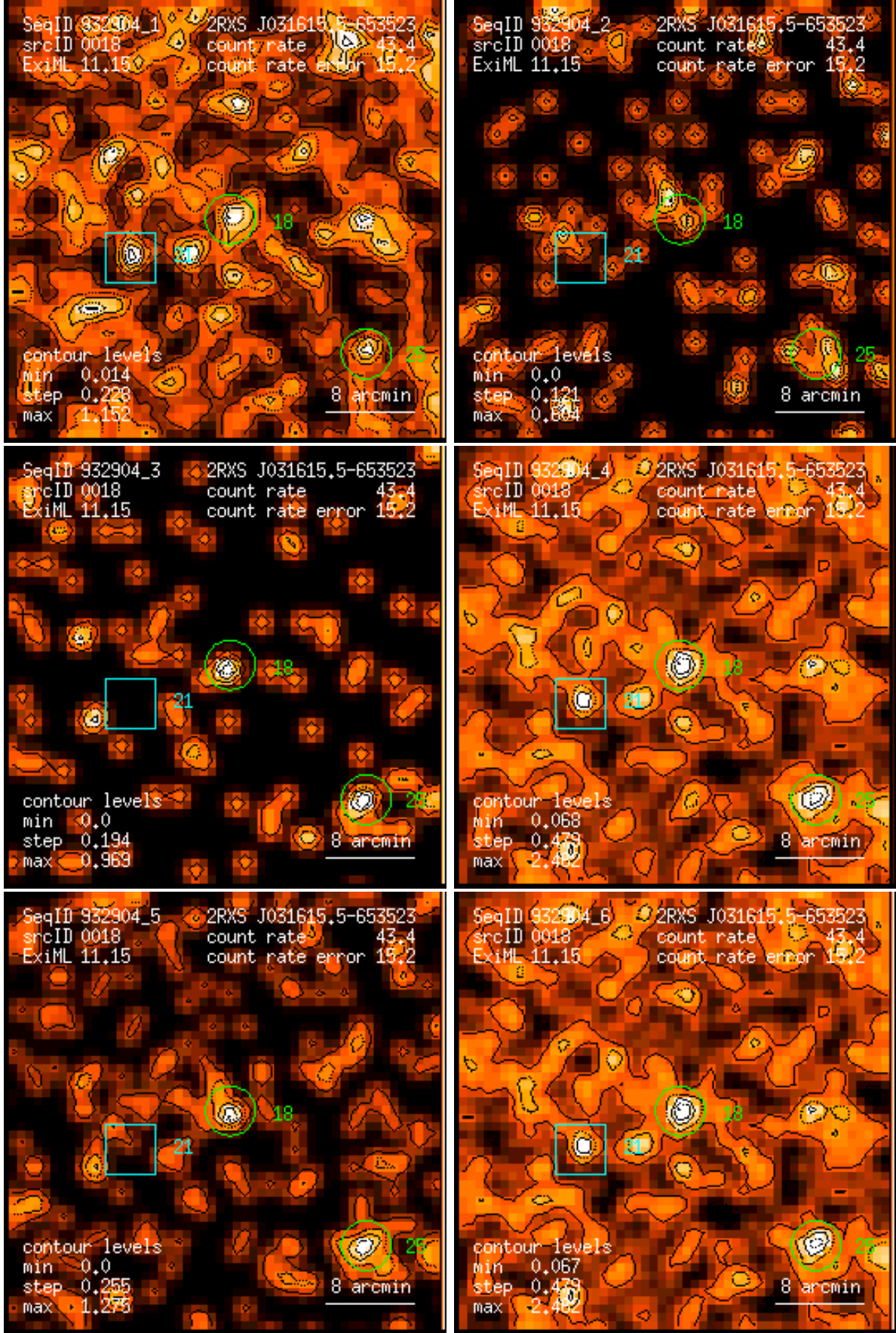
Figure 18: RASS 932904: detection 0018: band rate images, Gaussian filter: (1) PSPC channels 11 – 41, (2) 52 – 90, (3) 91 – 201, (4) 11 – 235, (5) 52 – 201, (6) 11 – 201. Broad band rates in counts/ks. Band rate contour levels in counts/ks/arcmin 2 .
