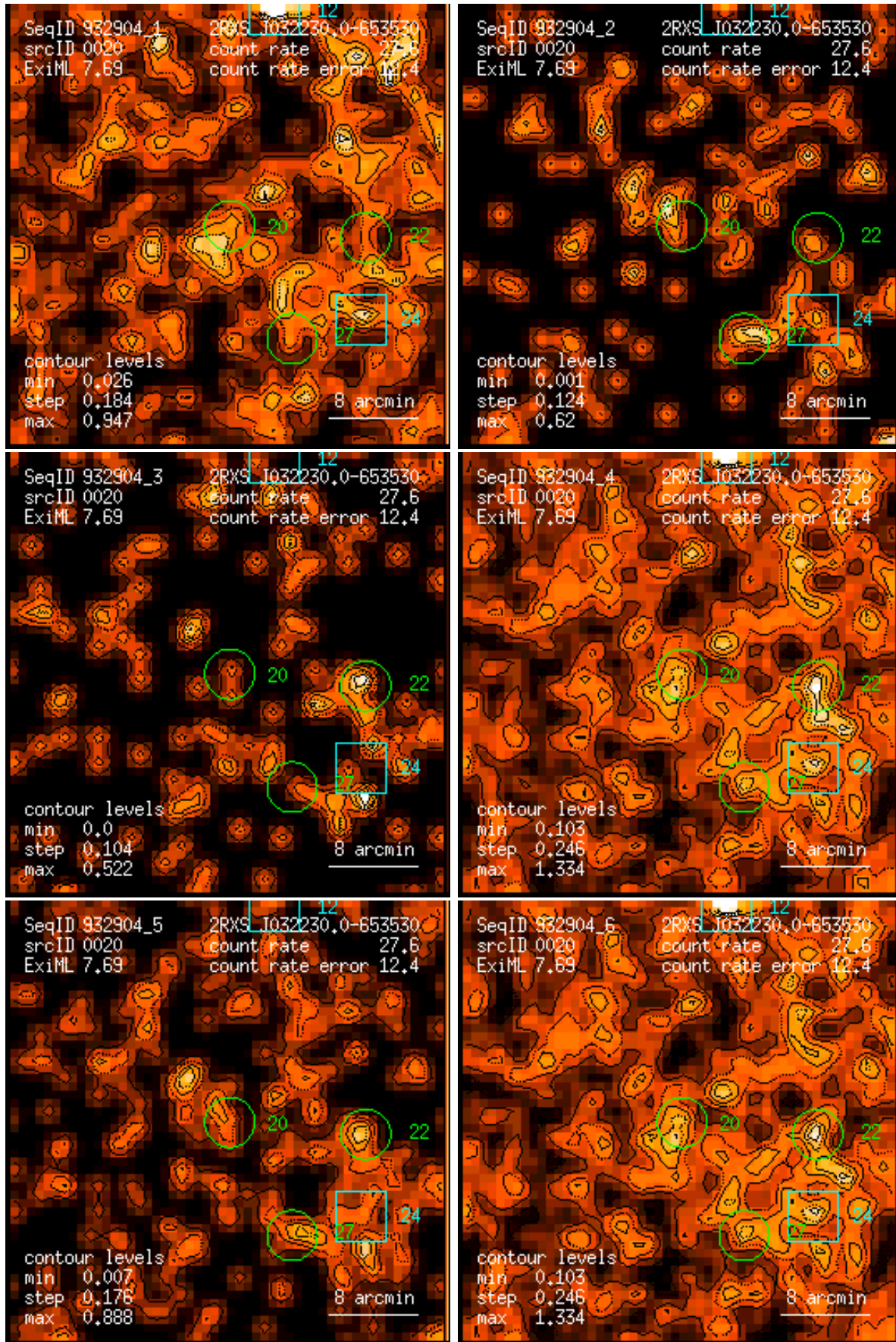
Figure 20: RASS 932904: detection 0020: band rate images, Gaussian filter: (1) PSPC channels 11 – 41, (2) 52 – 90, (3) 91 – 201, (4) 11 – 235, (5) 52 – 201, (6) 11 – 201. Broad band rates in counts/ks. Band rate contour levels in counts/ks/arcmin 2 .
