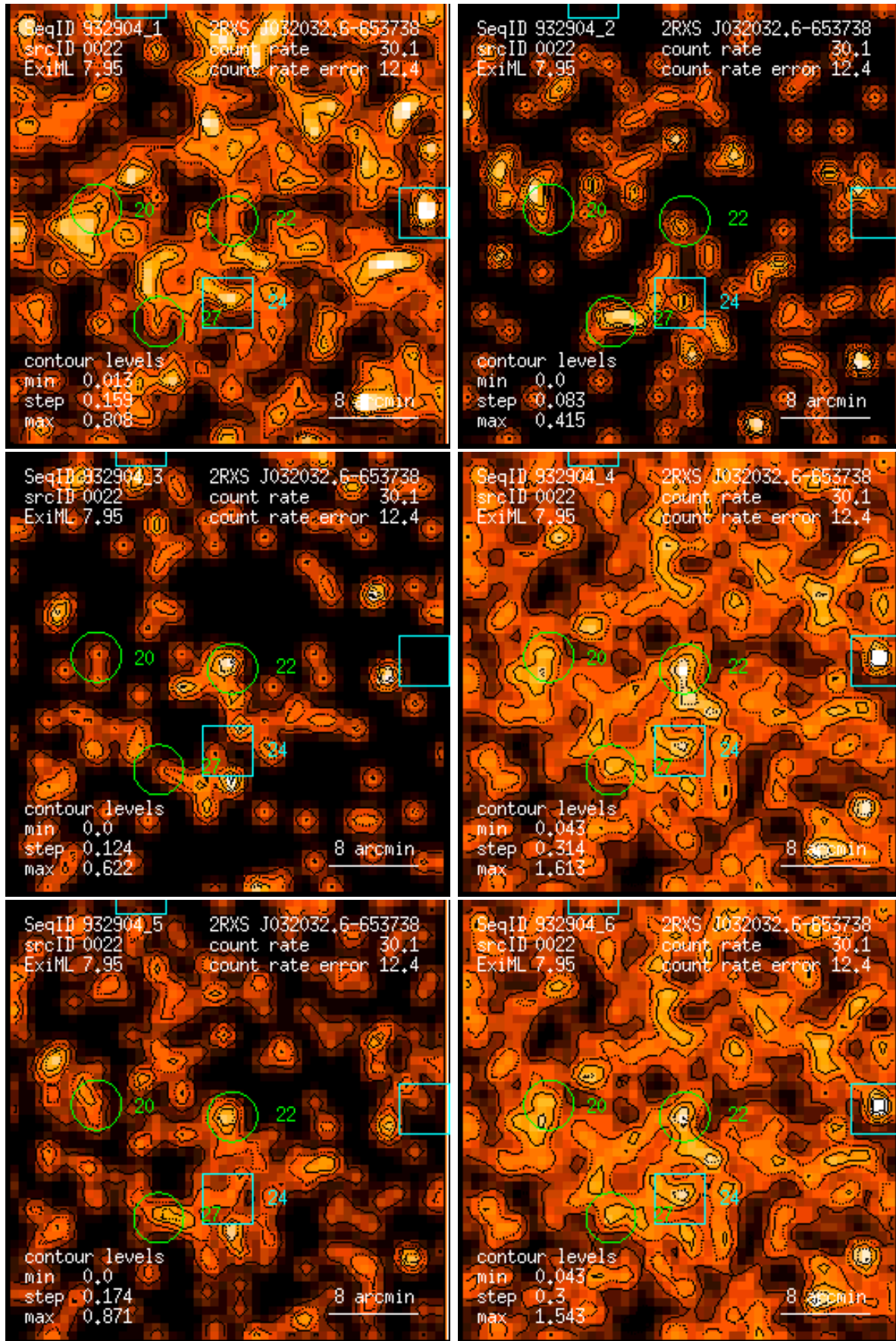
Figure 22: RASS 932904: detection 0022: band rate images, Gaussian filter: (1) PSPC channels 11 – 41, (2) 52 – 90, (3) 91 – 201, (4) 11 – 235, (5) 52 – 201, (6) 11 – 201. Broad band rates in counts/ks. Band rate contour levels in counts/ks/arcmin 2 .
