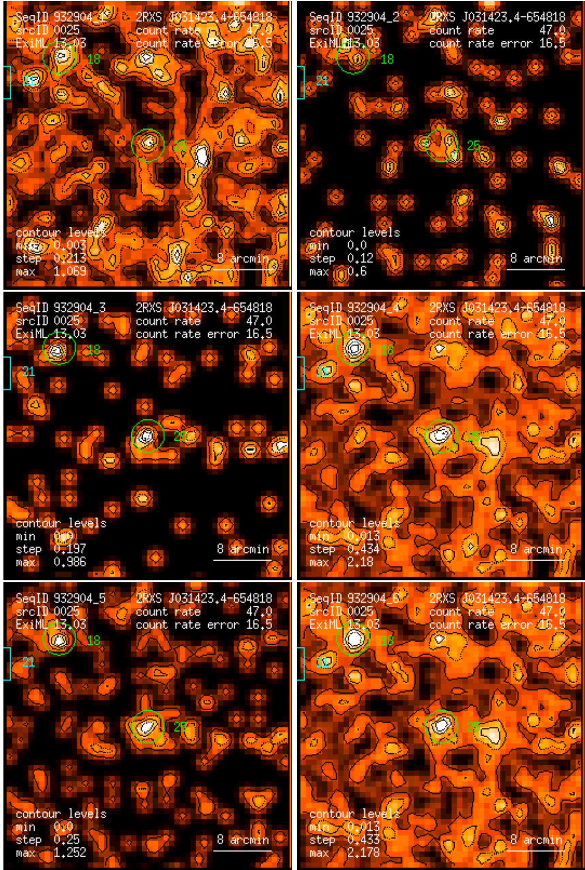
Figure 25: RASS 932904: detection 0025: band rate images, Gaussian filter: (1) PSPC channels 11 – 41, (2) 52 – 90, (3) 91 – 201, (4) 11 – 235, (5) 52 – 201, (6) 11 – 201. Broad band rates in counts/ks. Band rate contour levels in counts/ks/arcmin 2 .
