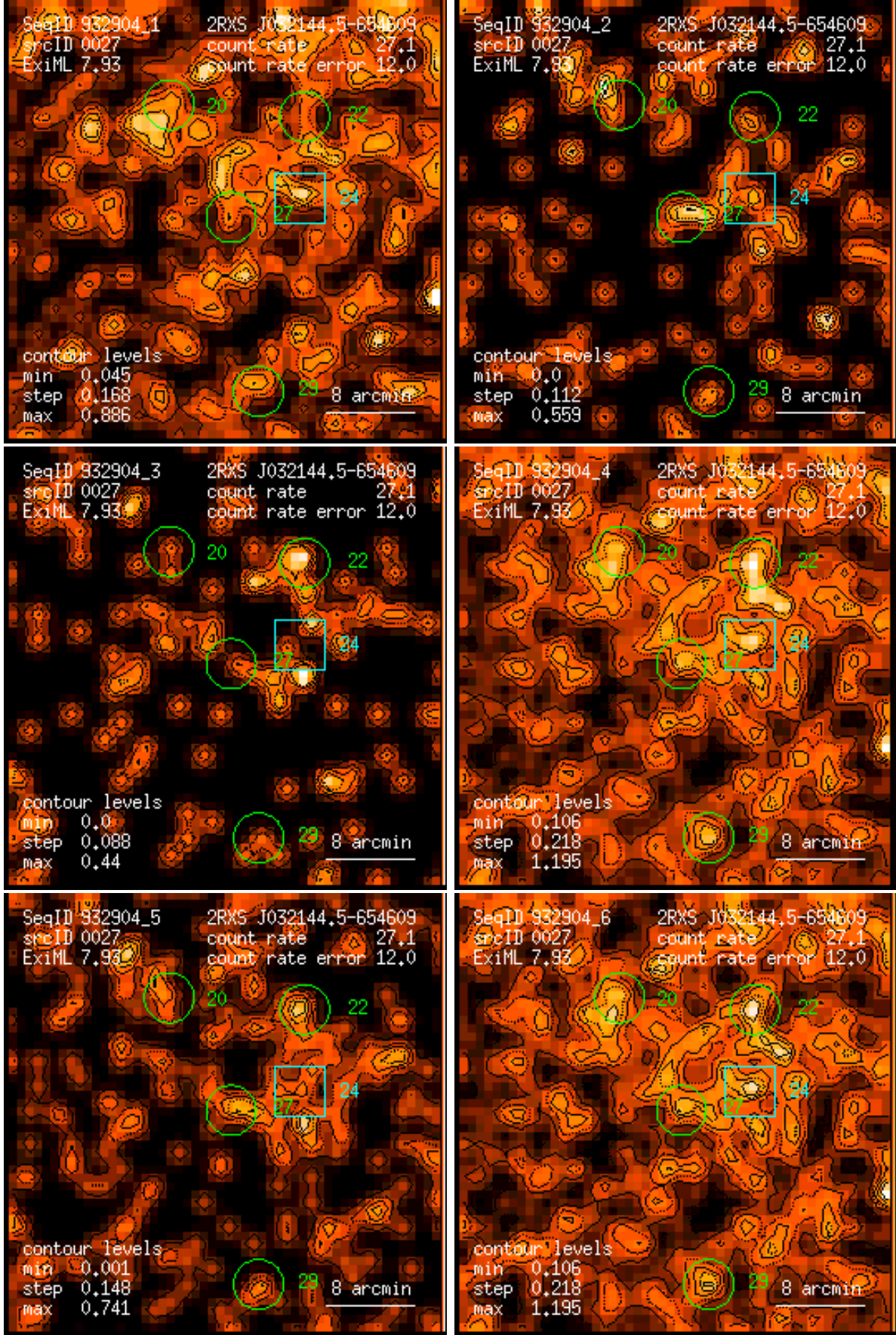
Figure 27: RASS 932904: detection 0027: band rate images, Gaussian filter: (1) PSPC channels 11 – 41, (2) 52 – 90, (3) 91 – 201, (4) 11 – 235, (5) 52 – 201, (6) 11 – 201. Broad band rates in counts/ks. Band rate contour levels in counts/ks/arcmin 2 .
