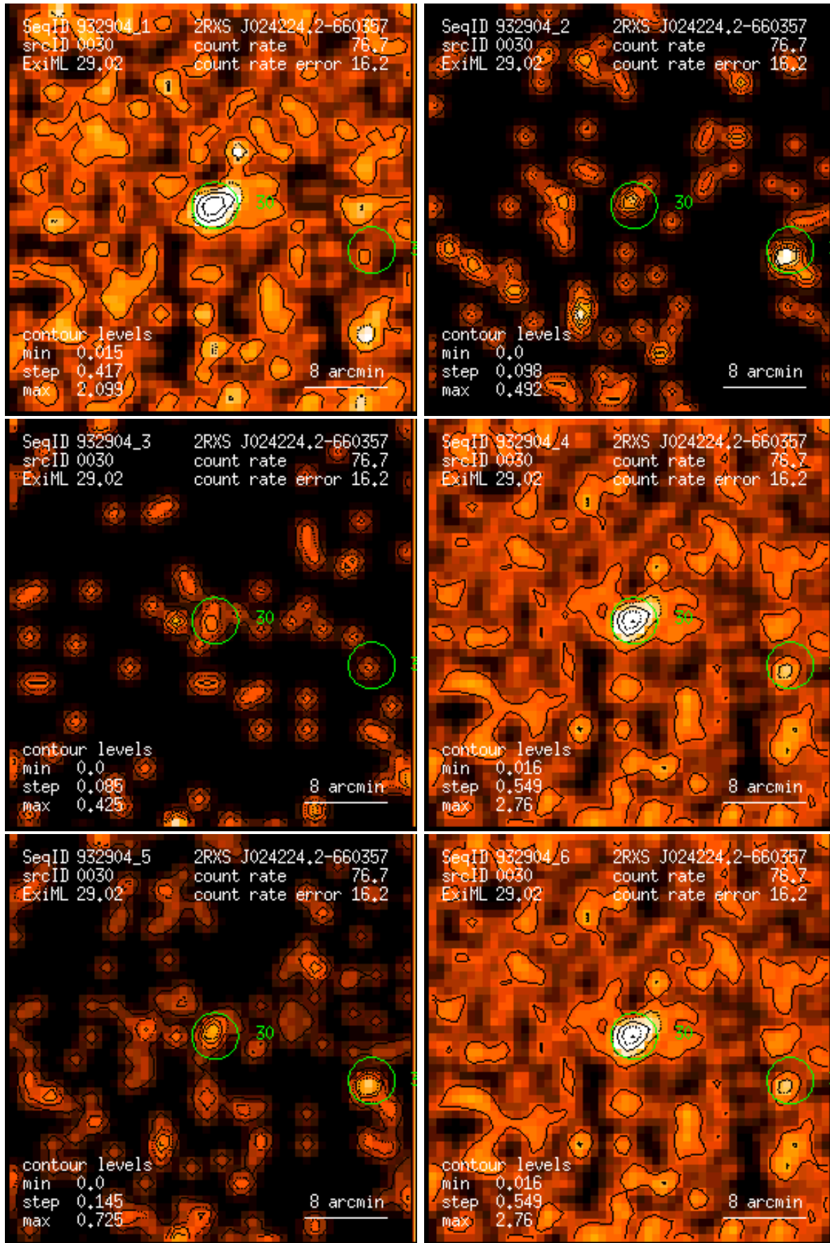
Figure 30: RASS 932904: detection 0030: band rate images, Gaussian filter: (1) PSPC channels 11 – 41, (2) 52 – 90, (3) 91 – 201, (4) 11 – 235, (5) 52 – 201, (6) 11 – 201. Broad band rates in counts/ks. Band rate contour levels in counts/ks/arcmin 2 .
