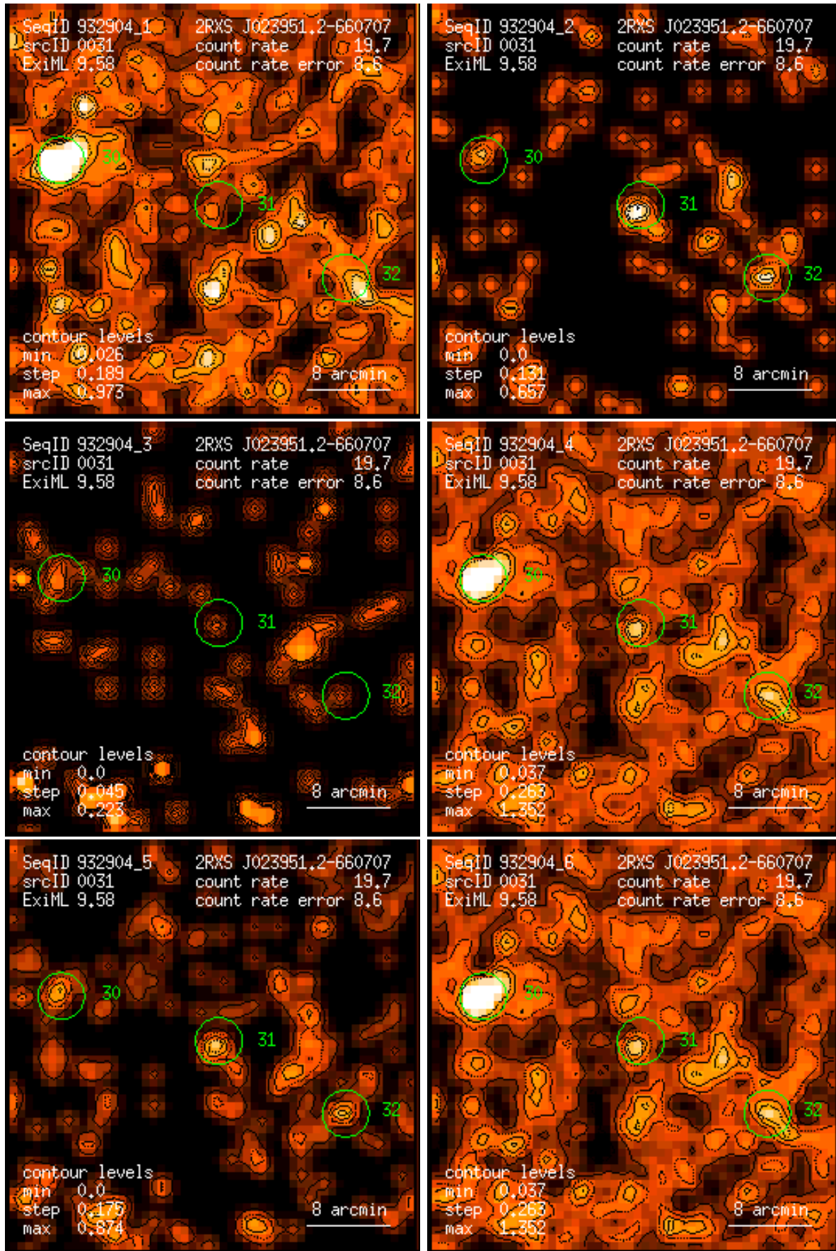
Figure 31: RASS 932904: detection 0031: band rate images, Gaussian filter: (1) PSPC channels 11 – 41, (2) 52 – 90, (3) 91 – 201, (4) 11 – 235, (5) 52 – 201, (6) 11 – 201. Broad band rates in counts/ks. Band rate contour levels in counts/ks/arcmin 2 .
