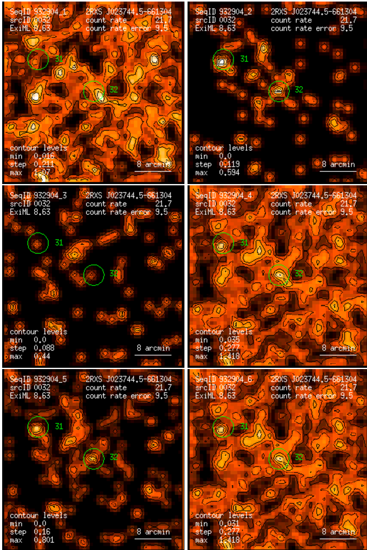
Figure 32: RASS 932904: detection 0032: band rate images, Gaussian filter: (1) PSPC channels 11 – 41, (2) 52 – 90, (3) 91 – 201, (4) 11 – 235, (5) 52 – 201, (6) 11 – 201. Broad band rates in counts/ks. Band rate contour levels in counts/ks/arcmin 2 .
