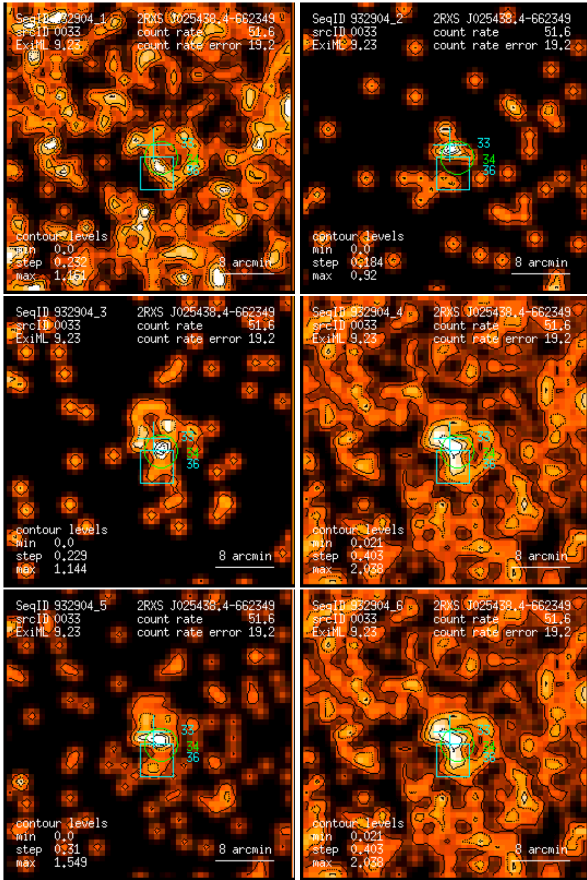
Figure 33: RASS 932904: detection 0033: band rate images, Gaussian filter: (1) PSPC channels 11 – 41, (2) 52 – 90, (3) 91 – 201, (4) 11 – 235, (5) 52 – 201, (6) 11 – 201. Broad band rates in counts/ks. Band rate contour levels in counts/ks/arcmin 2 .
