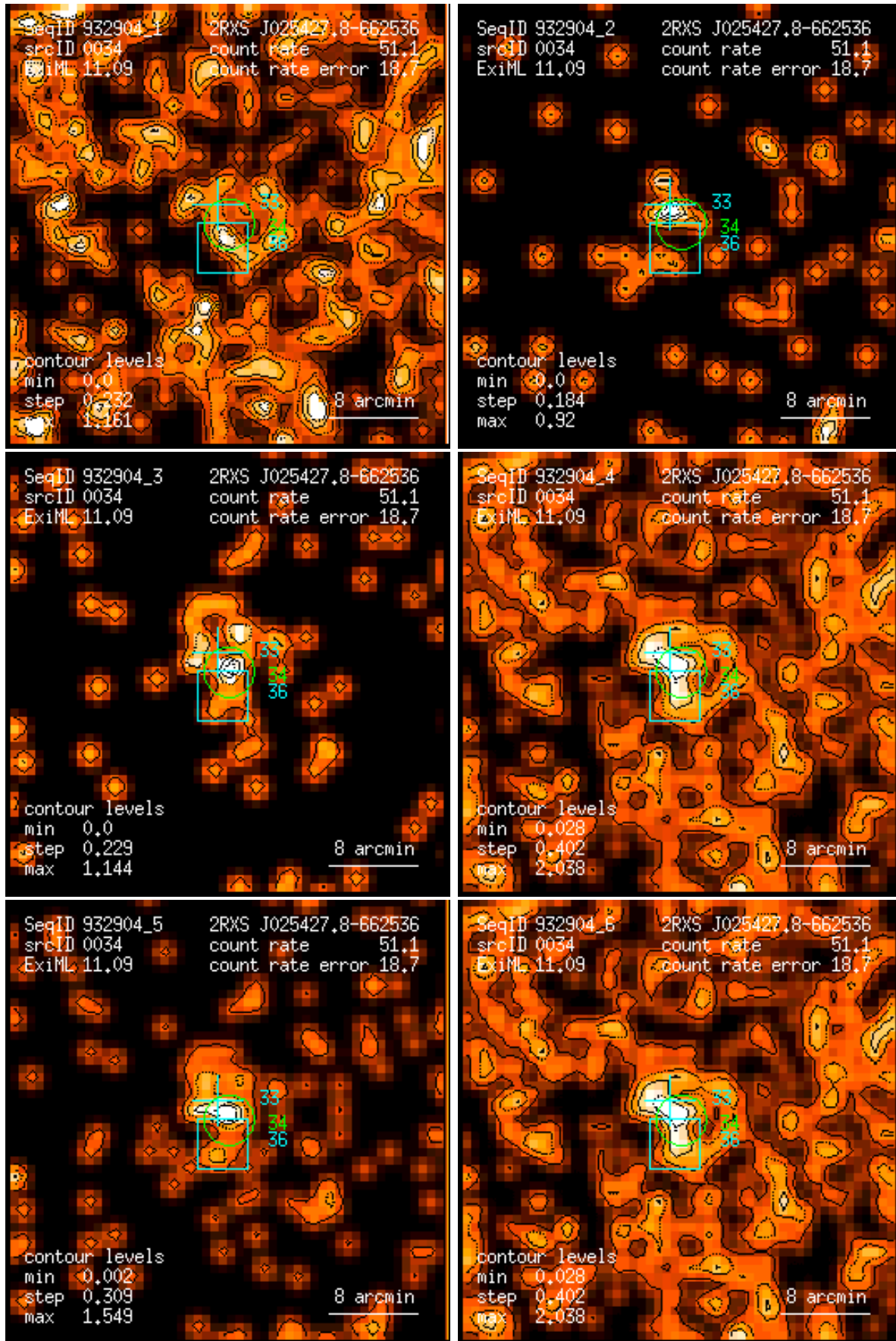
Figure 34: RASS 932904: detection 0034: band rate images, Gaussian filter: (1) PSPC channels 11 – 41, (2) 52 – 90, (3) 91 – 201, (4) 11 – 235, (5) 52 – 201, (6) 11 – 201. Broad band rates in counts/ks. Band rate contour levels in counts/ks/arcmin 2 .
