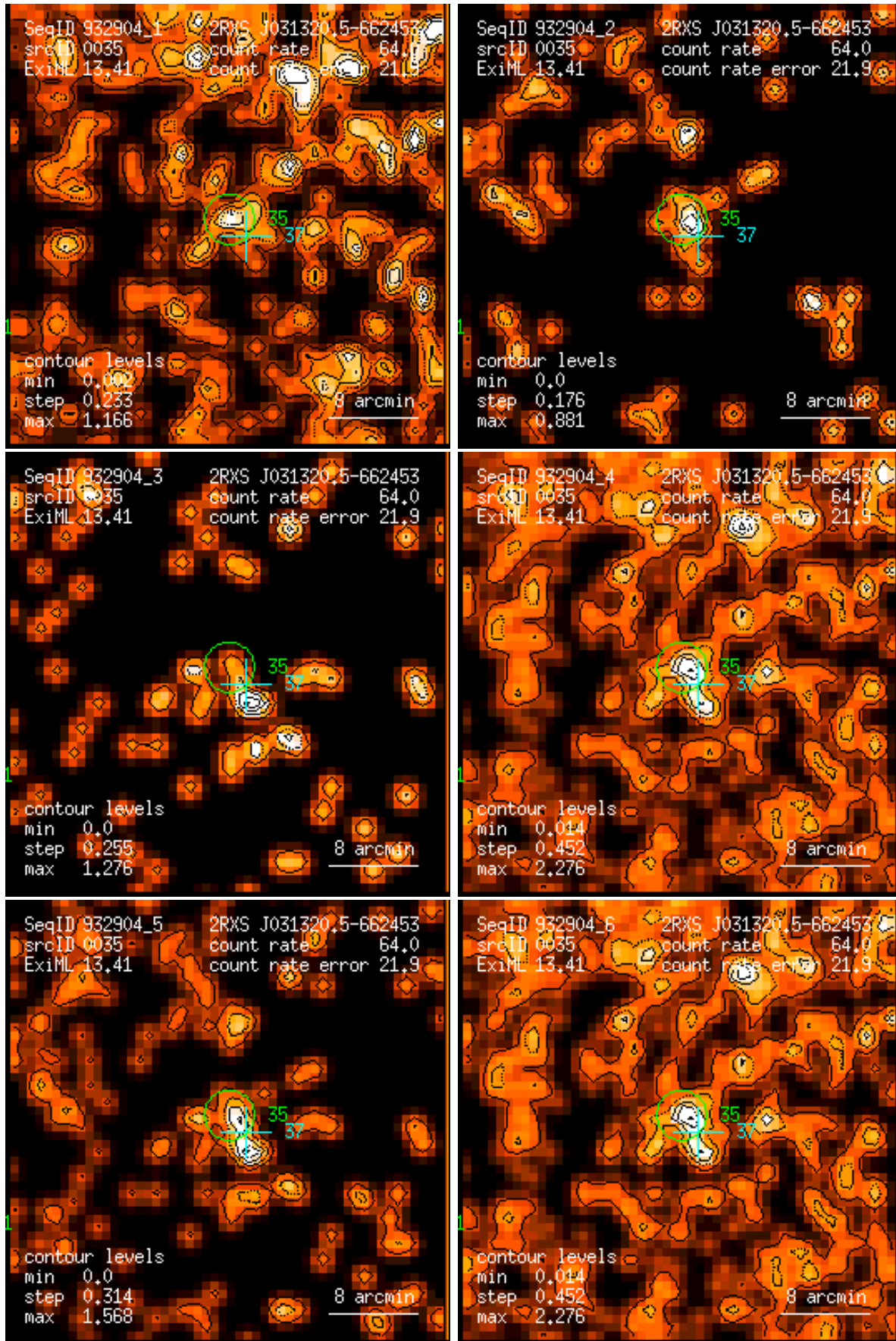
Figure 35: RASS 932904: detection 0035: band rate images, Gaussian filter: (1) PSPC channels 11 – 41, (2) 52 – 90, (3) 91 – 201, (4) 11 – 235, (5) 52 – 201, (6) 11 – 201. Broad band rates in counts/ks. Band rate contour levels in counts/ks/arcmin 2 .
