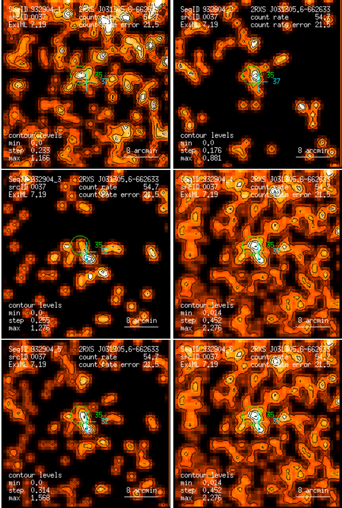
Figure 37: RASS 932904: detection 0037: band rate images, Gaussian filter: (1) PSPC channels 11 – 41, (2) 52 – 90, (3) 91 – 201, (4) 11 – 235, (5) 52 – 201, (6) 11 – 201. Broad band rates in counts/ks. Band rate contour levels in counts/ks/arcmin 2 .
