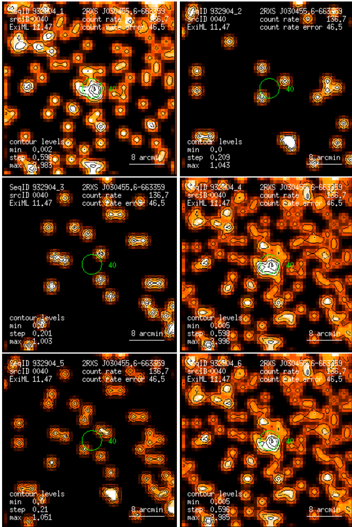
Figure 40: RASS 932904: detection 0040: band rate images, Gaussian filter: (1) PSPC channels 11 – 41, (2) 52 – 90, (3) 91 – 201, (4) 11 – 235, (5) 52 – 201, (6) 11 – 201. Broad band rates in counts/ks. Band rate contour levels in counts/ks/arcmin 2 .
