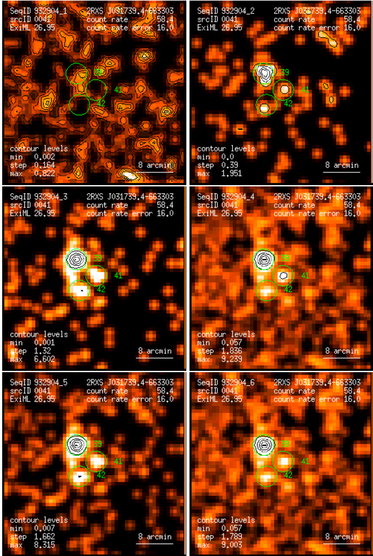
Figure 41: RASS 932904: detection 0041: band rate images, Gaussian filter: (1) PSPC channels 11 – 41, (2) 52 – 90, (3) 91 – 201, (4) 11 – 235, (5) 52 – 201, (6) 11 – 201. Broad band rates in counts/ks. Band rate contour levels in counts/ks/arcmin 2 .
