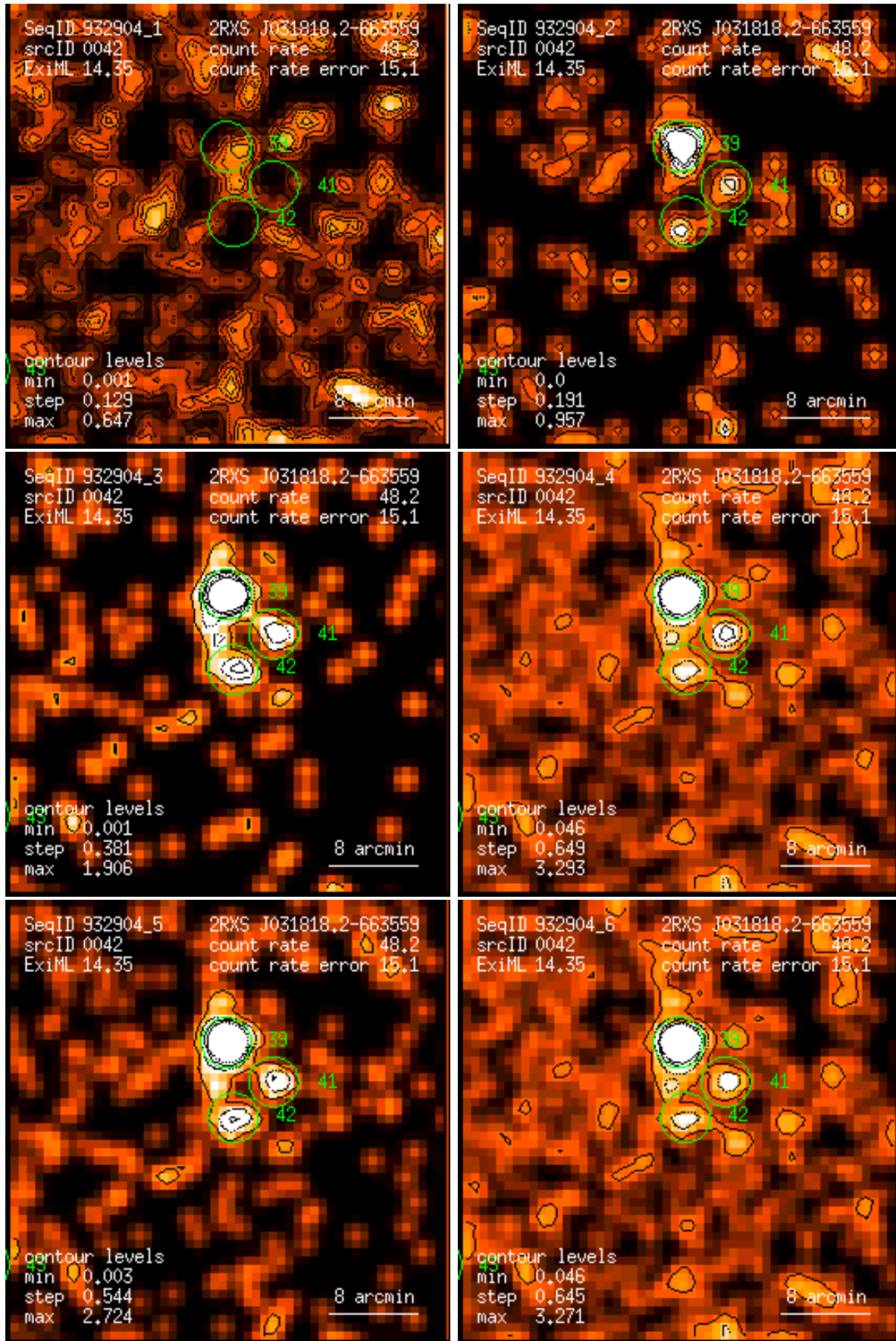
Figure 42: RASS 932904: detection 0042: band rate images, Gaussian filter: (1) PSPC channels 11 – 41, (2) 52 – 90, (3) 91 – 201, (4) 11 – 235, (5) 52 – 201, (6) 11 – 201. Broad band rates in counts/ks. Band rate contour levels in counts/ks/arcmin 2 .
