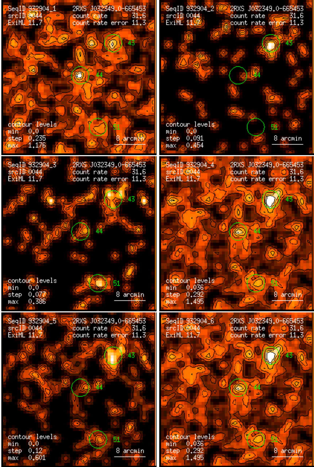
Figure 44: RASS 932904: detection 0044: band rate images, Gaussian filter: (1) PSPC channels 11 – 41, (2) 52 – 90, (3) 91 – 201, (4) 11 – 235, (5) 52 – 201, (6) 11 – 201. Broad band rates in counts/ks. Band rate contour levels in counts/ks/arcmin 2 .
