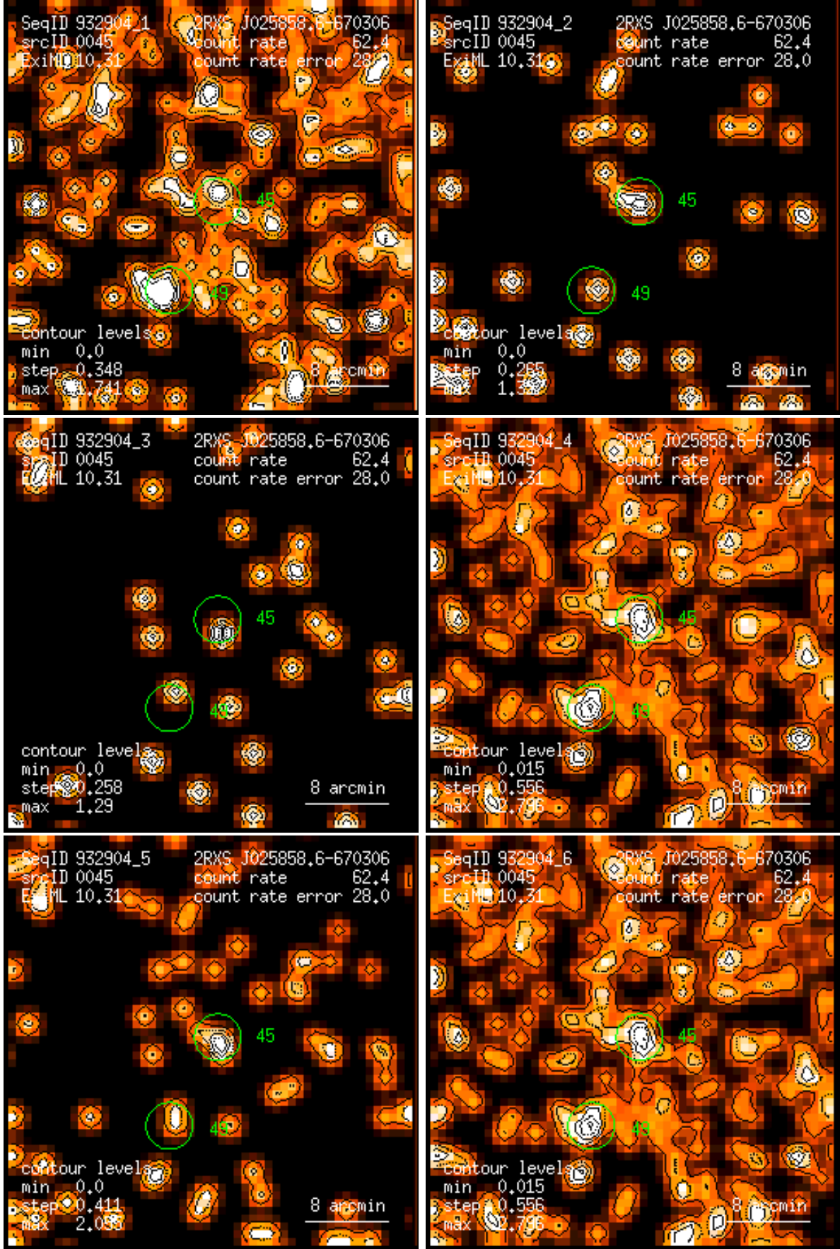
Figure 45: RASS 932904: detection 0045: band rate images, Gaussian filter: (1) PSPC channels 11 – 41, (2) 52 – 90, (3) 91 – 201, (4) 11 – 235, (5) 52 – 201, (6) 11 – 201. Broad band rates in counts/ks. Band rate contour levels in counts/ks/arcmin 2 .
