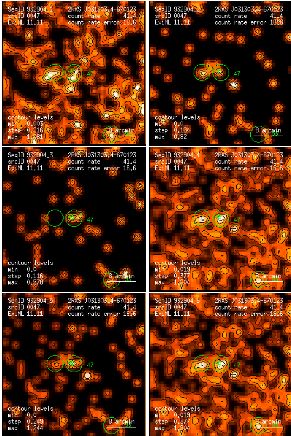
Figure 47: RASS 932904: detection 0047: band rate images, Gaussian filter: (1) PSPC channels 11 – 41, (2) 52 – 90, (3) 91 – 201, (4) 11 – 235, (5) 52 – 201, (6) 11 – 201. Broad band rates in counts/ks. Band rate contour levels in counts/ks/arcmin 2 .
