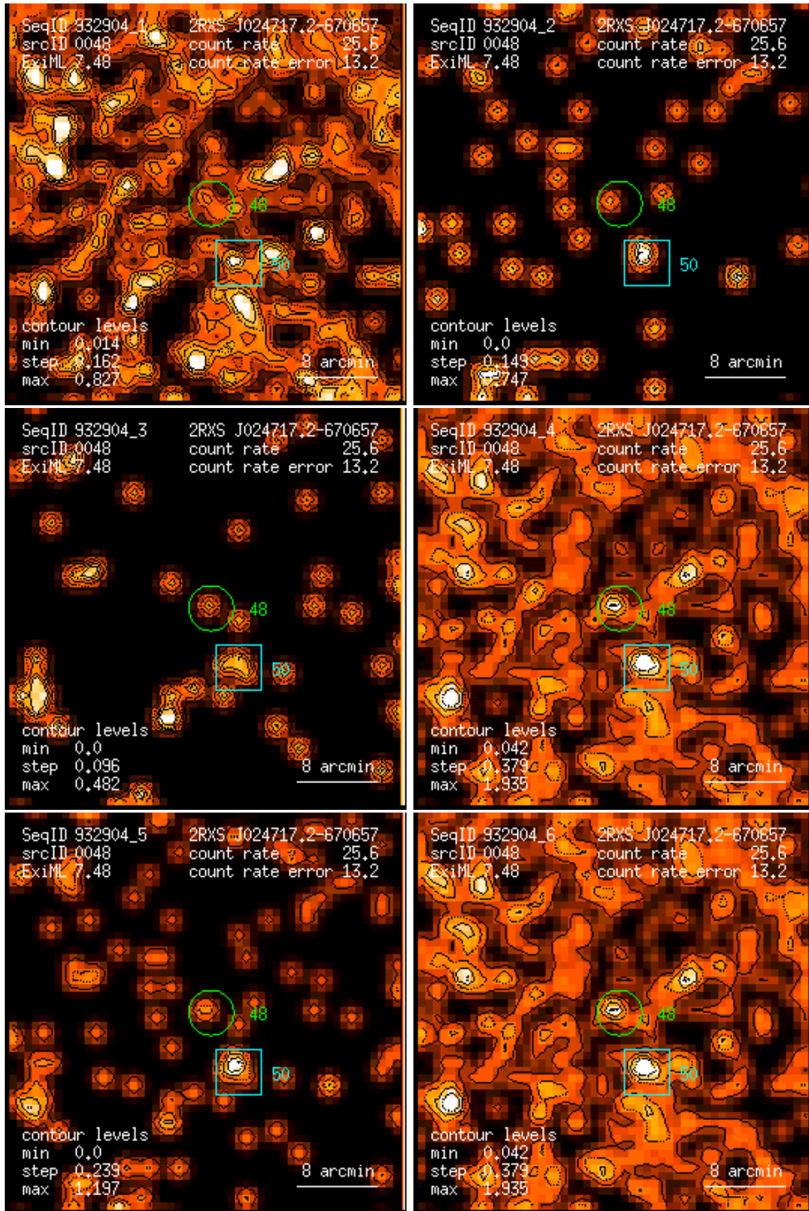
Figure 48: RASS 932904: detection 0048: band rate images, Gaussian filter: (1) PSPC channels 11 – 41, (2) 52 – 90, (3) 91 – 201, (4) 11 – 235, (5) 52 – 201, (6) 11 – 201. Broad band rates in counts/ks. Band rate contour levels in counts/ks/arcmin 2 .
