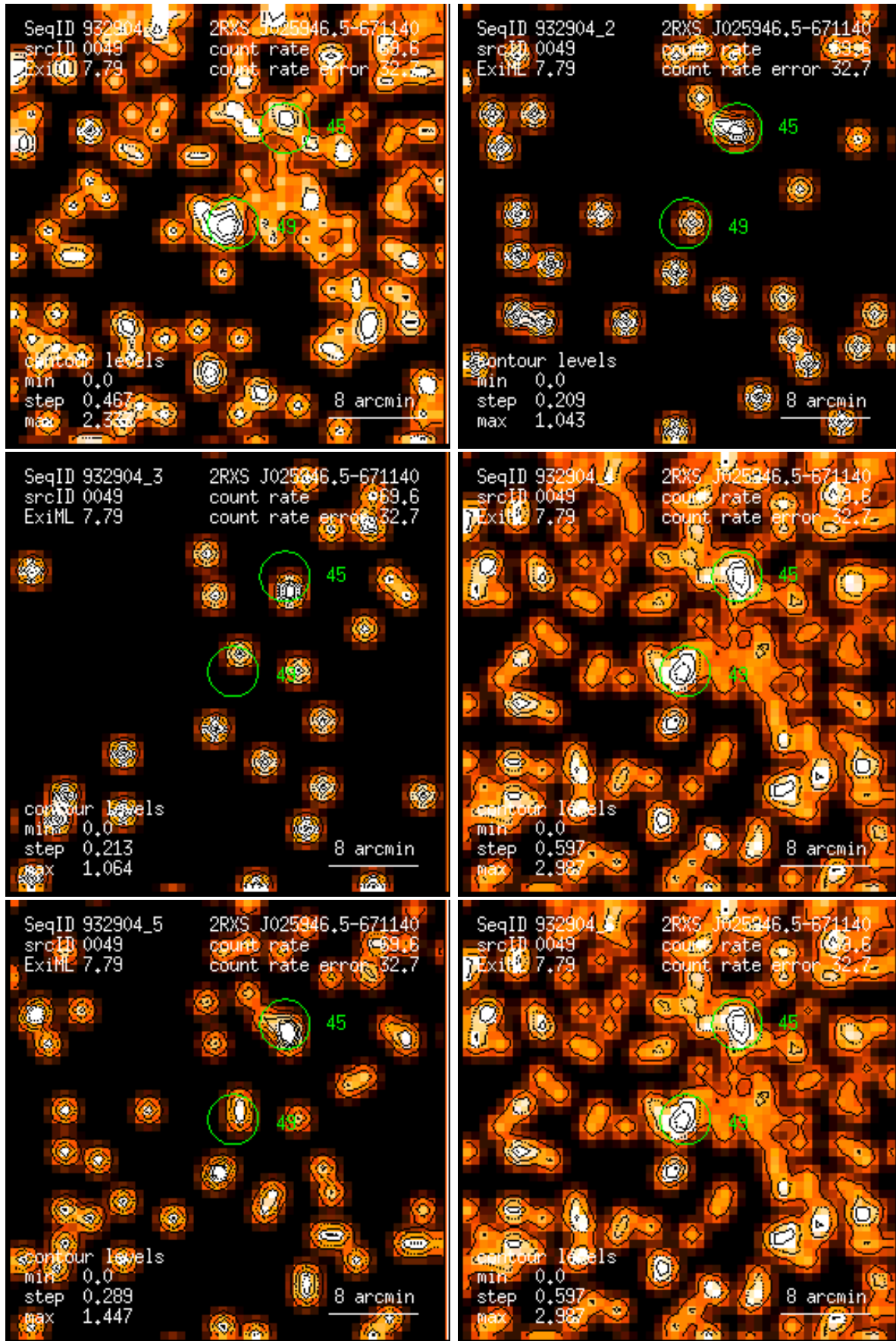
Figure 49: RASS 932904: detection 0049: band rate images, Gaussian filter: (1) PSPC channels 11 – 41, (2) 52 – 90, (3) 91 – 201, (4) 11 – 235, (5) 52 – 201, (6) 11 – 201. Broad band rates in counts/ks. Band rate contour levels in counts/ks/arcmin 2 .
