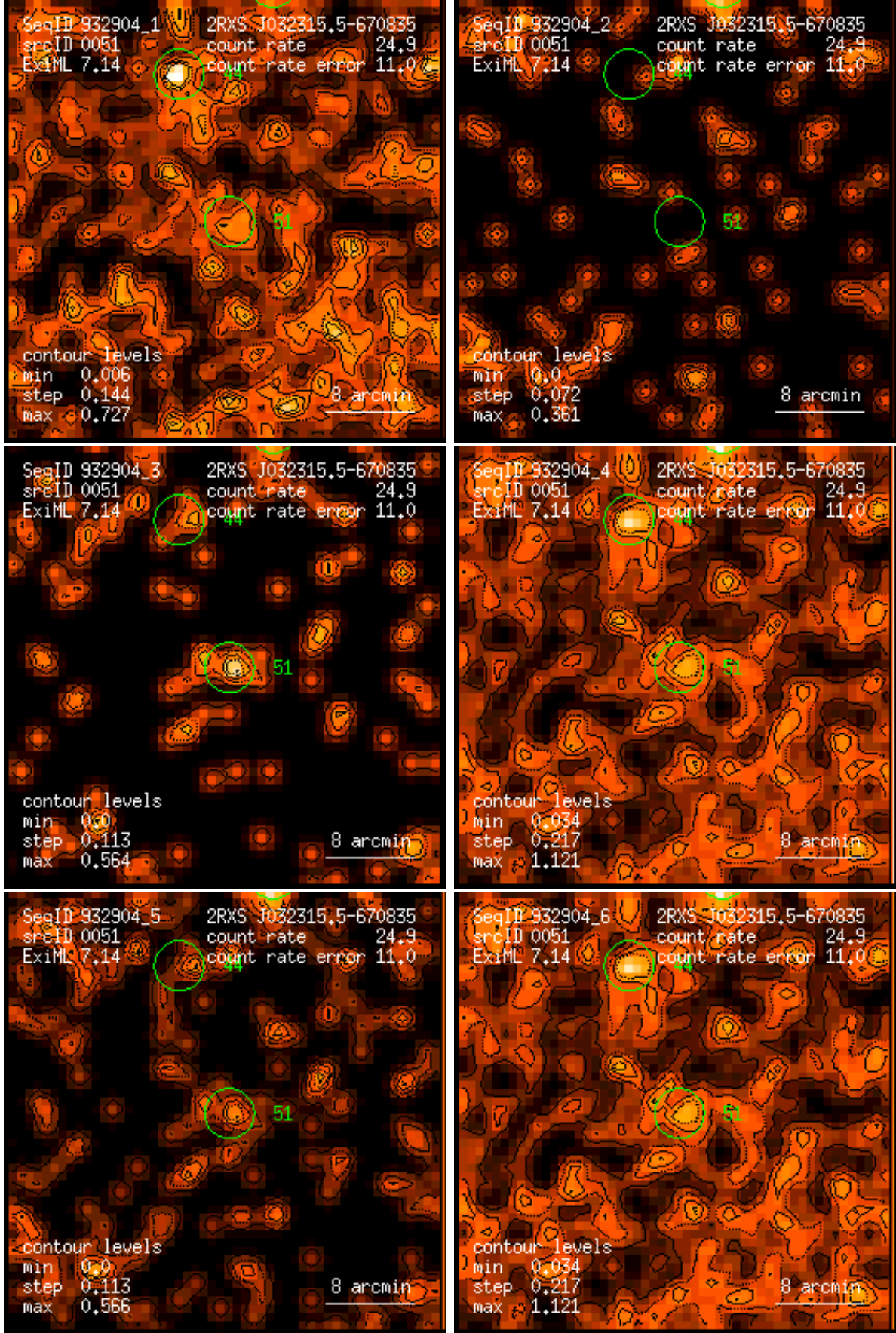
Figure 51: RASS 932904: detection 0051: band rate images, Gaussian filter: (1) PSPC channels 11 – 41, (2) 52 – 90, (3) 91 – 201, (4) 11 – 235, (5) 52 – 201, (6) 11 – 201. Broad band rates in counts/ks. Band rate contour levels in counts/ks/arcmin 2 .
