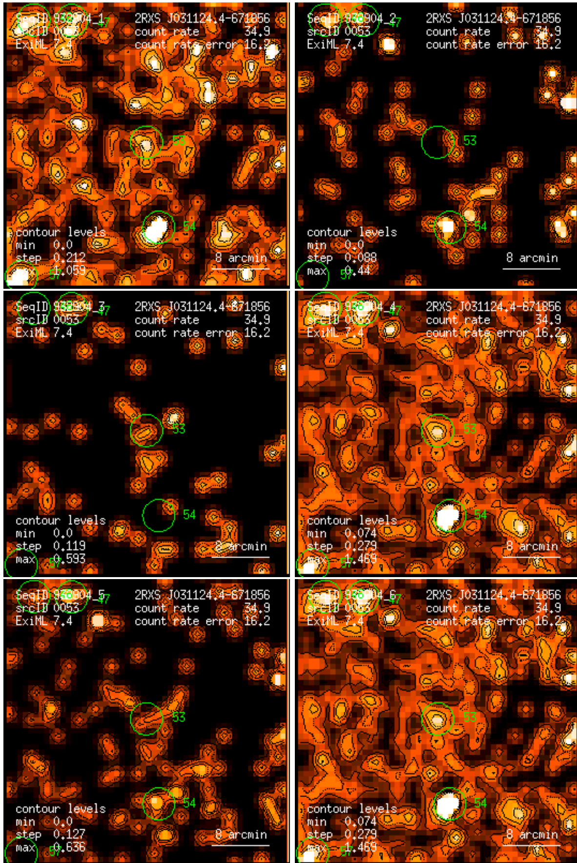
Figure 53: RASS 932904: detection 0053: band rate images, Gaussian filter: (1) PSPC channels 11 – 41, (2) 52 – 90, (3) 91 – 201, (4) 11 – 235, (5) 52 – 201, (6) 11 – 201. Broad band rates in counts/ks. Band rate contour levels in counts/ks/arcmin 2 .
