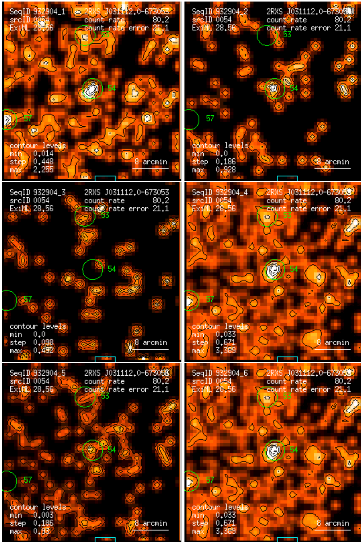
Figure 54: RASS 932904: detection 0054: band rate images, Gaussian filter: (1) PSPC channels 11 – 41, (2) 52 – 90, (3) 91 – 201, (4) 11 – 235, (5) 52 – 201, (6) 11 – 201. Broad band rates in counts/ks. Band rate contour levels in counts/ks/arcmin 2 .
