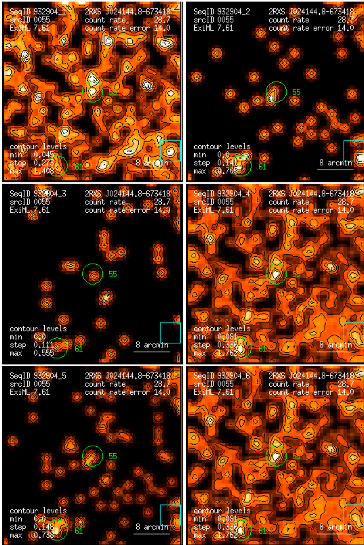
Figure 55: RASS 932904: detection 0055: band rate images, Gaussian filter: (1) PSPC channels 11 – 41, (2) 52 – 90, (3) 91 – 201, (4) 11 – 235, (5) 52 – 201, (6) 11 – 201. Broad band rates in counts/ks. Band rate contour levels in counts/ks/arcmin 2 .
