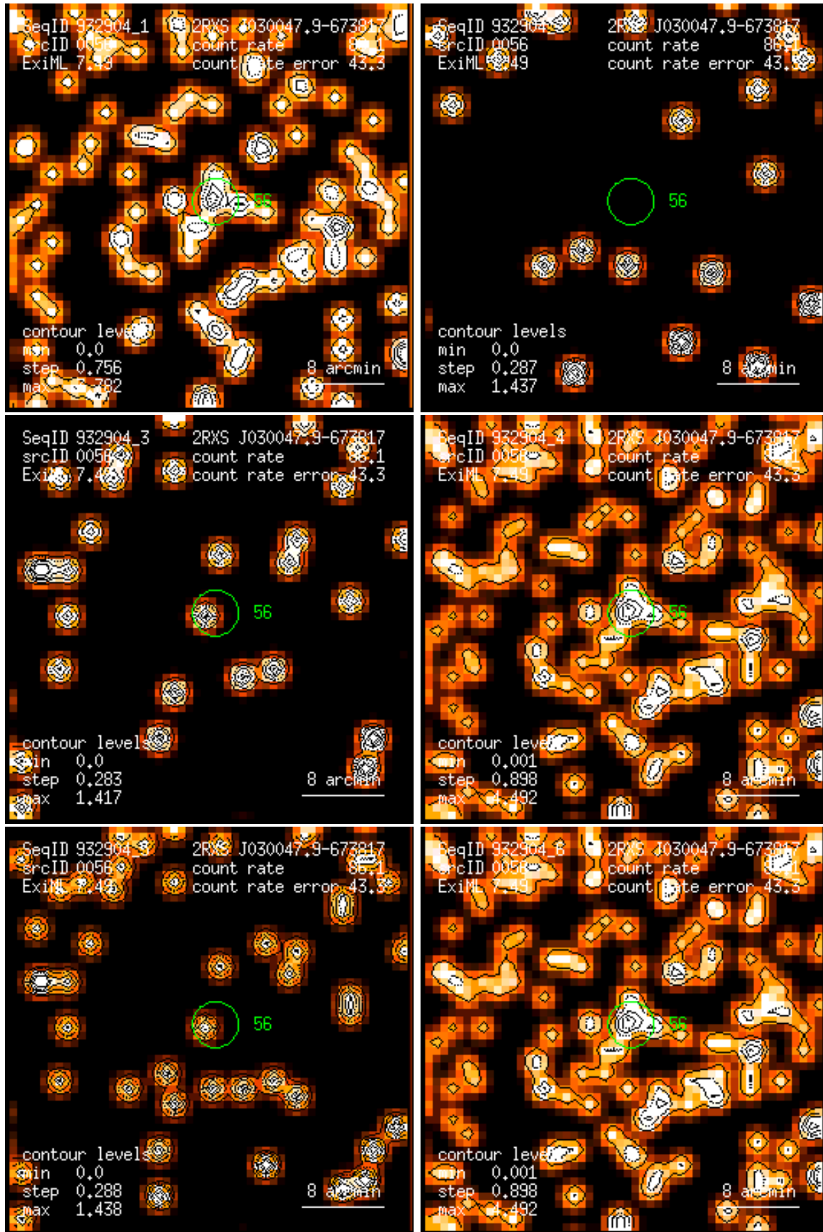
Figure 56: RASS 932904: detection 0056: band rate images, Gaussian filter: (1) PSPC channels 11 – 41, (2) 52 – 90, (3) 91 – 201, (4) 11 – 235, (5) 52 – 201, (6) 11 – 201. Broad band rates in counts/ks. Band rate contour levels in counts/ks/arcmin 2 .
