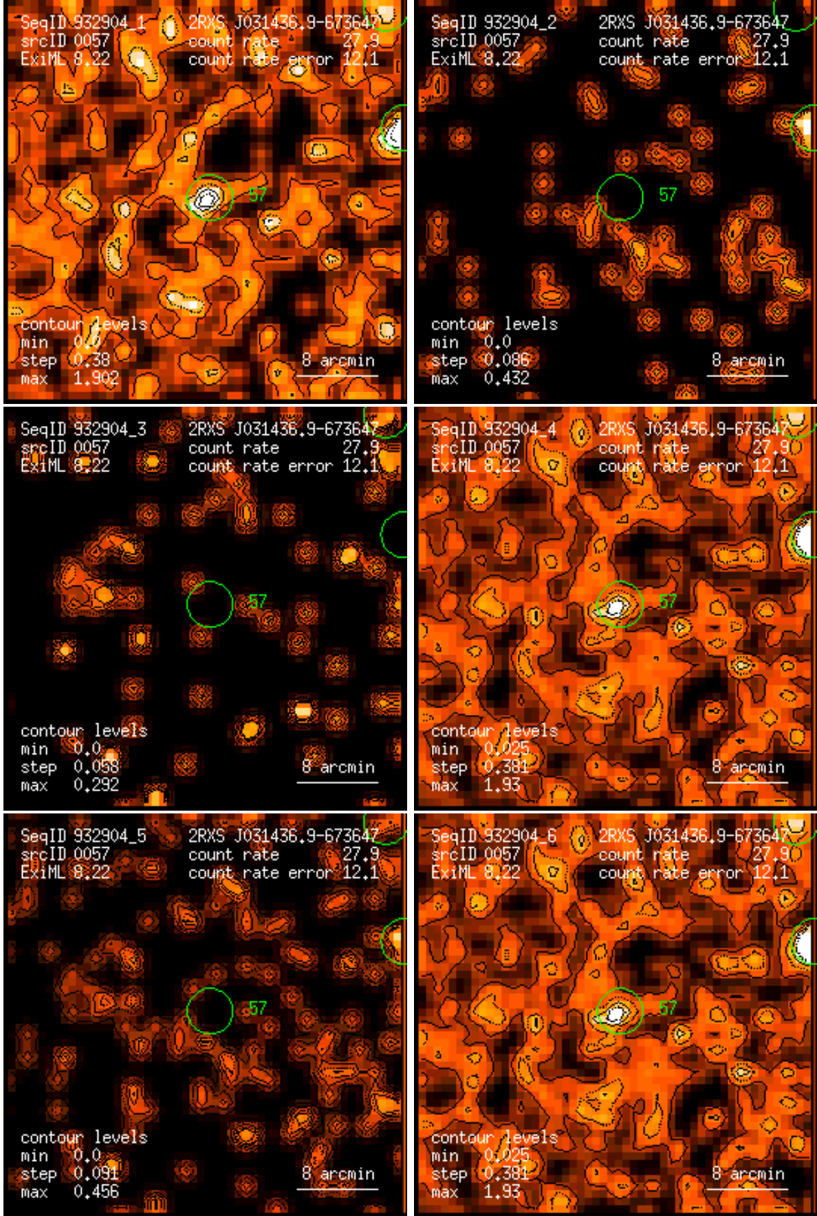
Figure 57: RASS 932904: detection 0057: band rate images, Gaussian filter: (1) PSPC channels 11 – 41, (2) 52 – 90, (3) 91 – 201, (4) 11 – 235, (5) 52 – 201, (6) 11 – 201. Broad band rates in counts/ks. Band rate contour levels in counts/ks/arcmin 2 .
