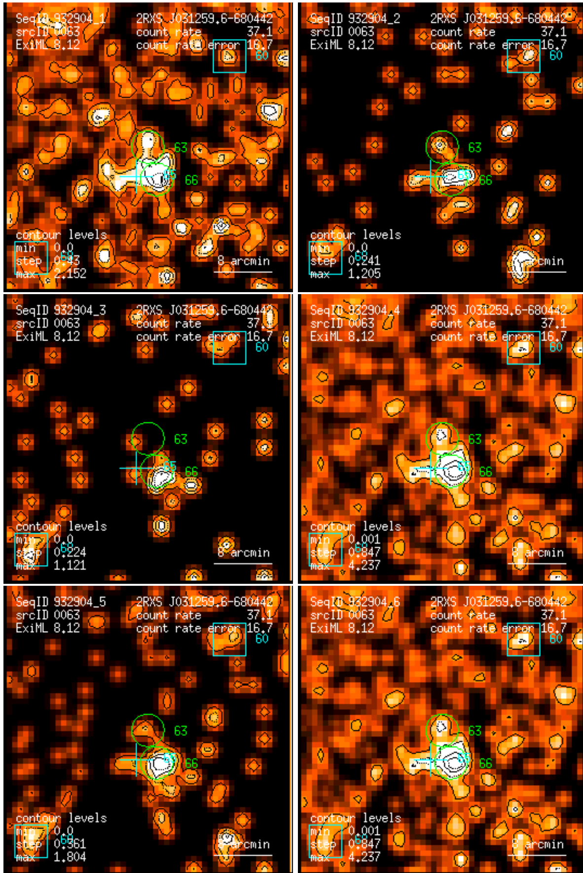
Figure 63: RASS 932904: detection 0063: band rate images, Gaussian filter: (1) PSPC channels 11 – 41, (2) 52 – 90, (3) 91 – 201, (4) 11 – 235, (5) 52 – 201, (6) 11 – 201. Broad band rates in counts/ks. Band rate contour levels in counts/ks/arcmin 2 .
