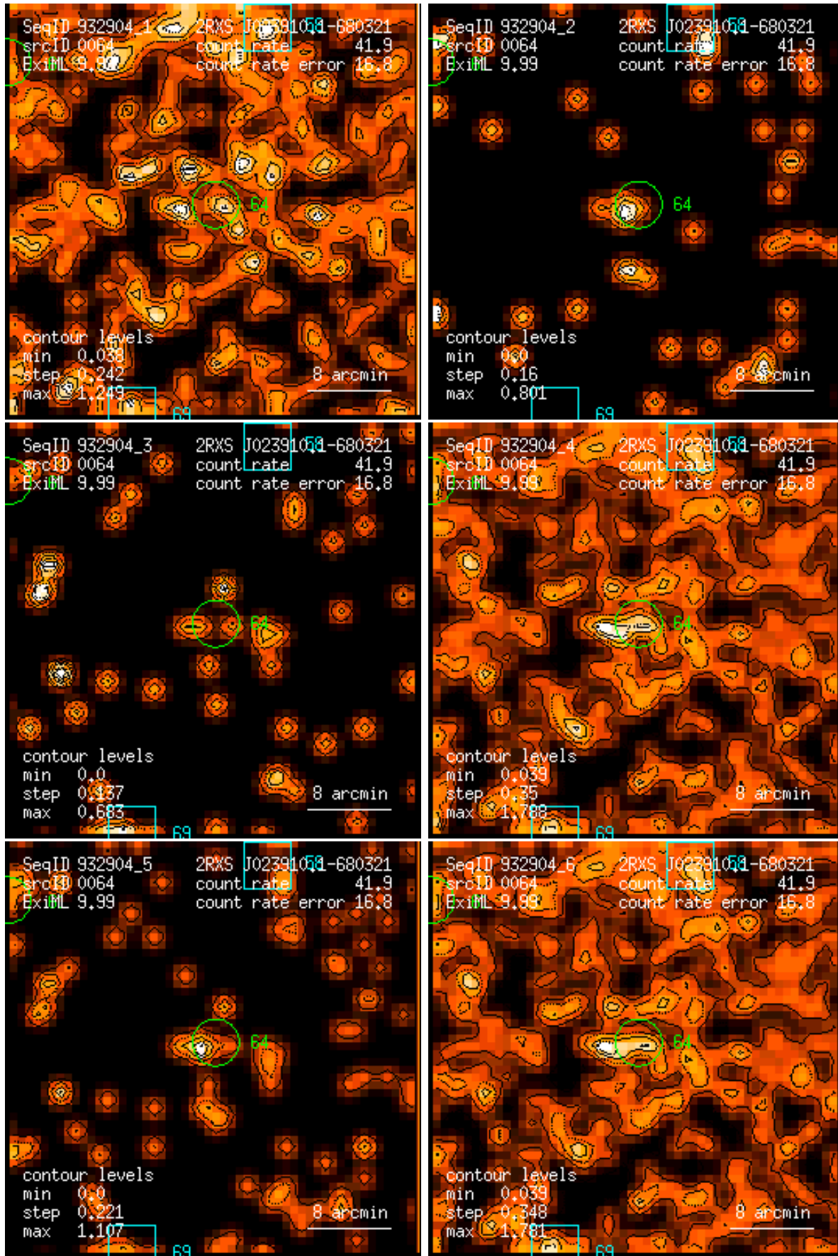
Figure 64: RASS 932904: detection 0064: band rate images, Gaussian filter: (1) PSPC channels 11 – 41, (2) 52 – 90, (3) 91 – 201, (4) 11 – 235, (5) 52 – 201, (6) 11 – 201. Broad band rates in counts/ks. Band rate contour levels in counts/ks/arcmin 2 .
