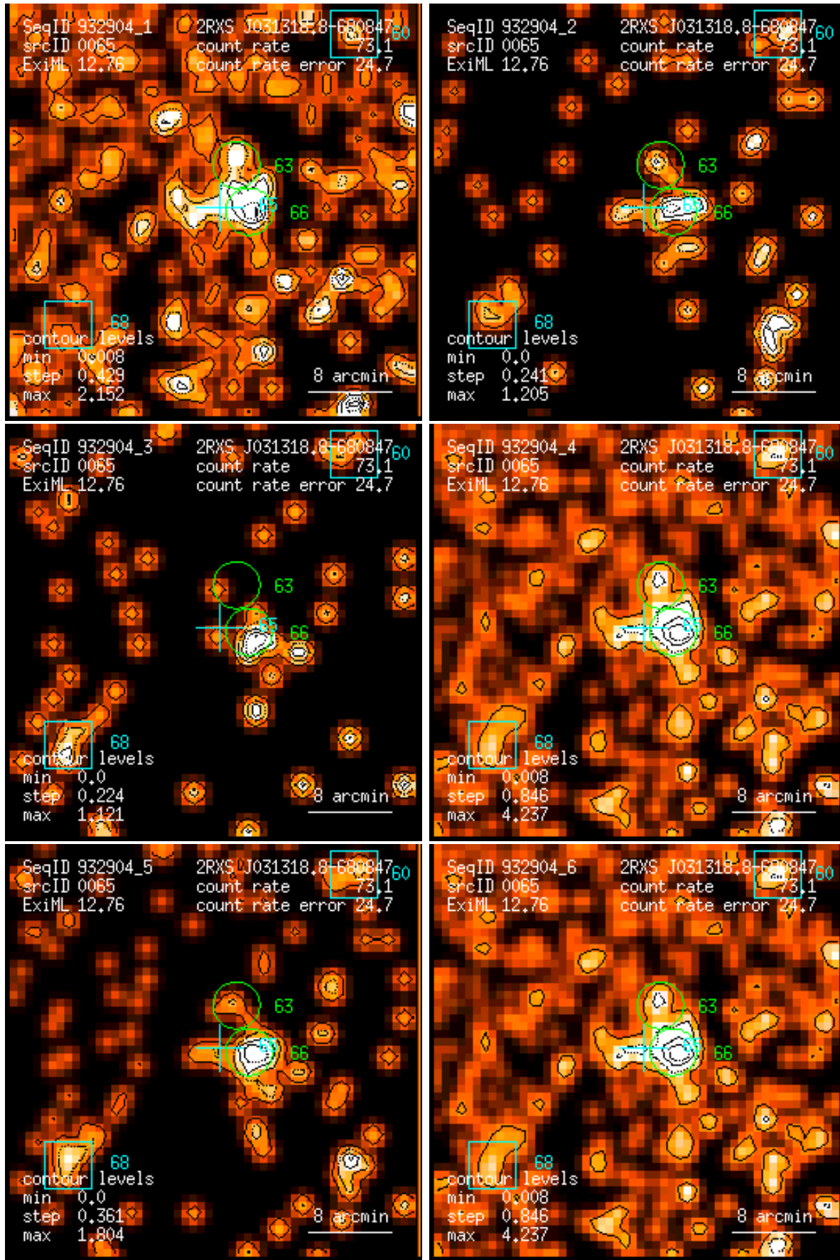
Figure 65: RASS 932904: detection 0065: band rate images, Gaussian filter: (1) PSPC channels 11 – 41, (2) 52 – 90, (3) 91 – 201, (4) 11 – 235, (5) 52 – 201, (6) 11 – 201. Broad band rates in counts/ks. Band rate contour levels in counts/ks/arcmin 2 .
