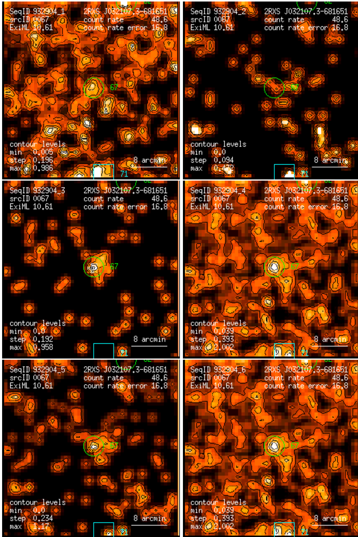
Figure 67: RASS 932904: detection 0067: band rate images, Gaussian filter: (1) PSPC channels 11 – 41, (2) 52 – 90, (3) 91 – 201, (4) 11 – 235, (5) 52 – 201, (6) 11 – 201. Broad band rates in counts/ks. Band rate contour levels in counts/ks/arcmin 2 .
