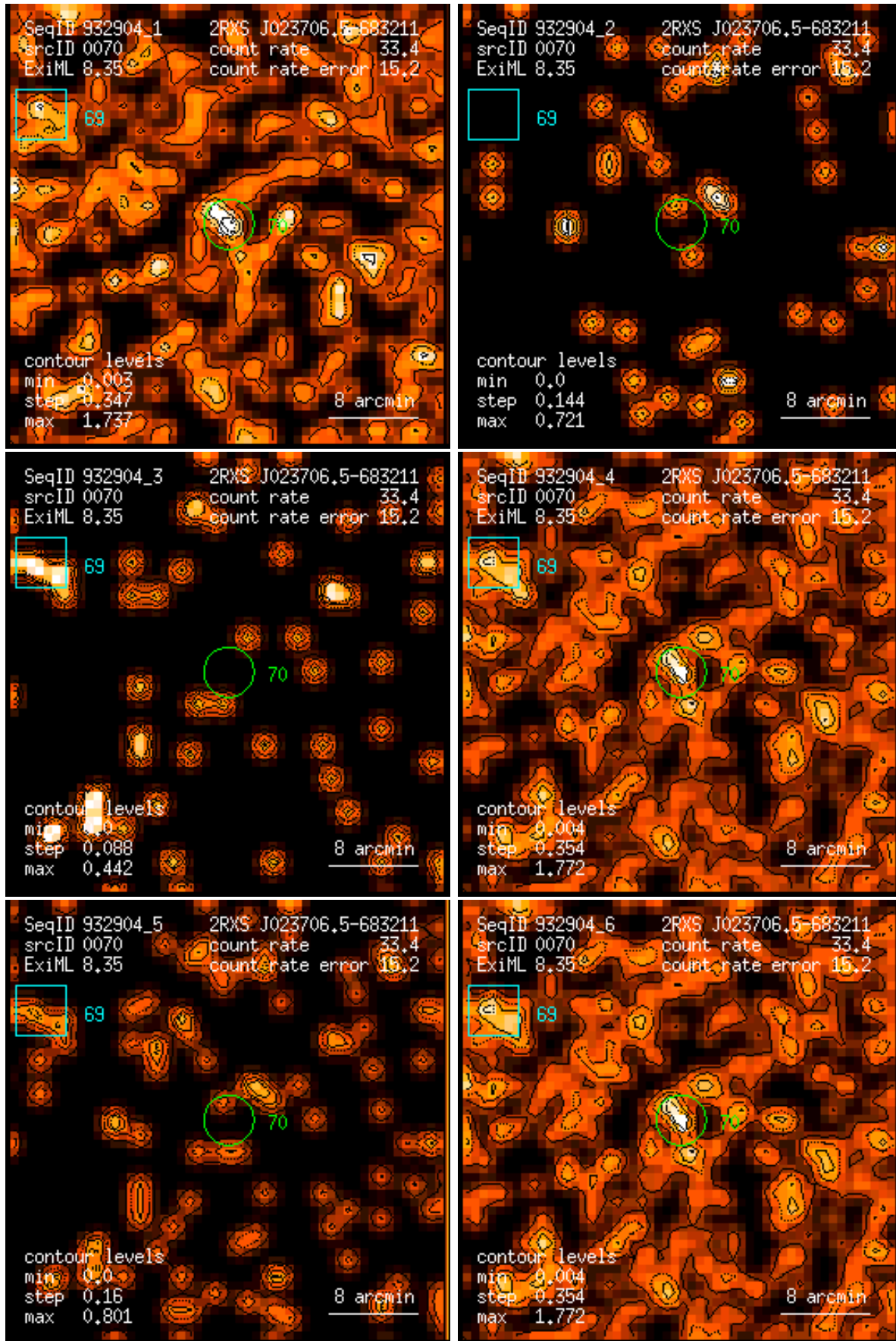
Figure 70: RASS 932904: detection 0070: band rate images, Gaussian filter: (1) PSPC channels 11 – 41, (2) 52 – 90, (3) 91 – 201, (4) 11 – 235, (5) 52 – 201, (6) 11 – 201. Broad band rates in counts/ks. Band rate contour levels in counts/ks/arcmin 2 .
