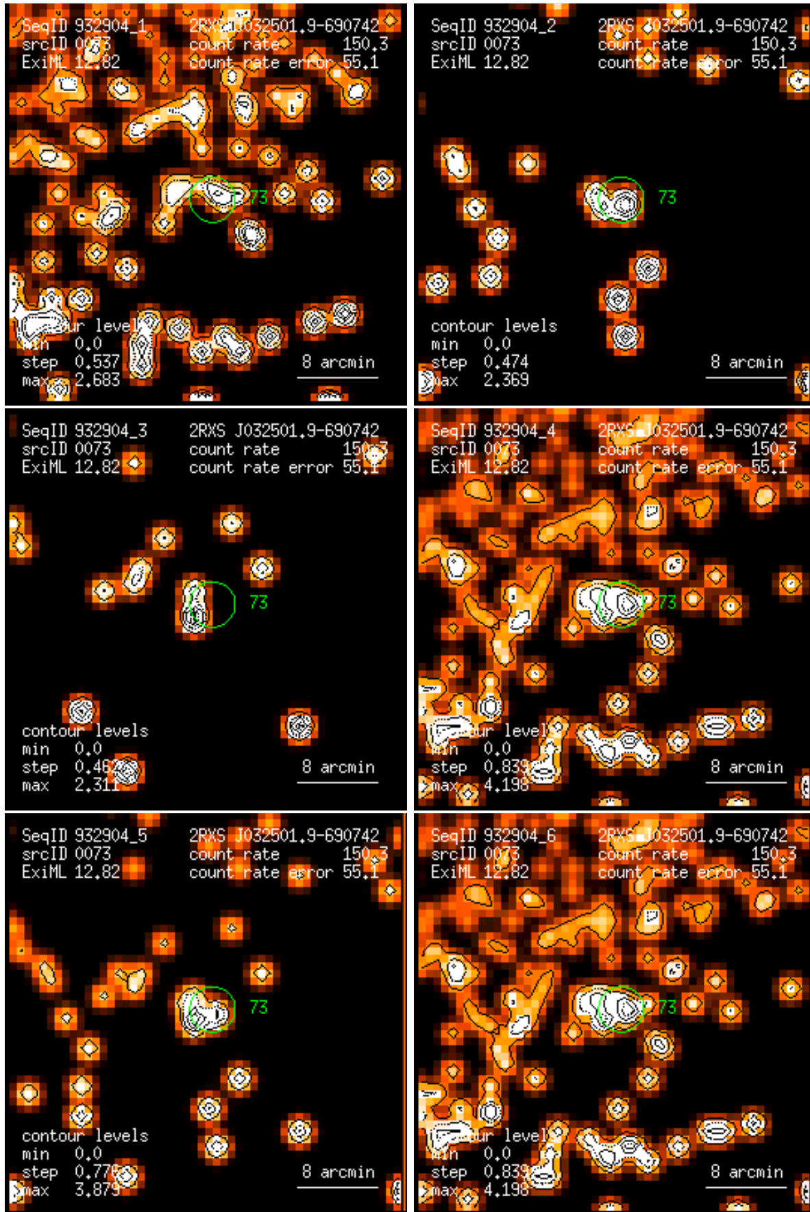
Figure 73: RASS 932904: detection 0073: band rate images, Gaussian filter: (1) PSPC channels 11 – 41, (2) 52 – 90, (3) 91 – 201, (4) 11 – 235, (5) 52 – 201, (6) 11 – 201. Broad band rates in counts/ks. Band rate contour levels in counts/ks/arcmin 2 .
