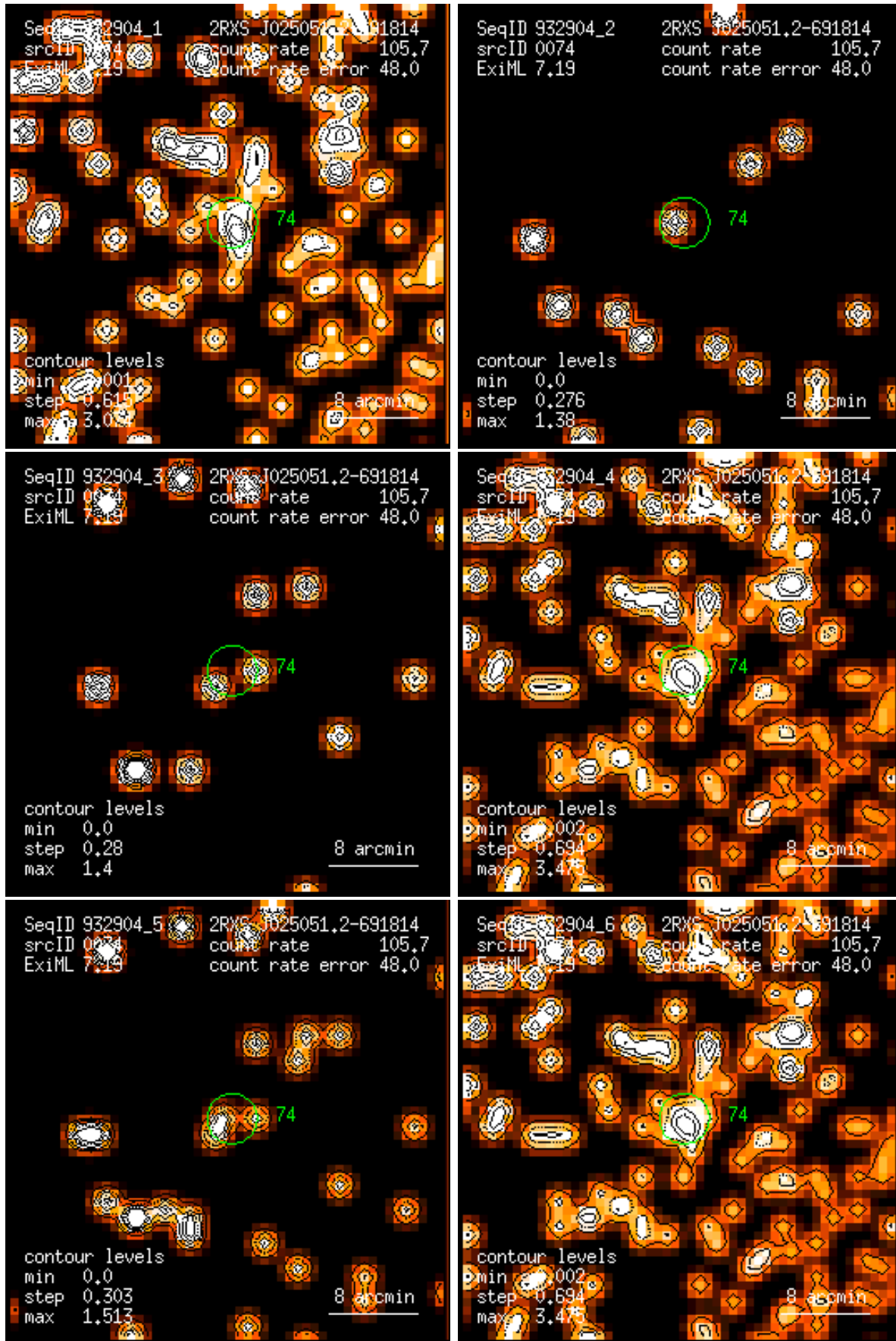
Figure 74: RASS 932904: detection 0074: band rate images, Gaussian filter: (1) PSPC channels 11 – 41, (2) 52 – 90, (3) 91 – 201, (4) 11 – 235, (5) 52 – 201, (6) 11 – 201. Broad band rates in counts/ks. Band rate contour levels in counts/ks/arcmin 2 .
