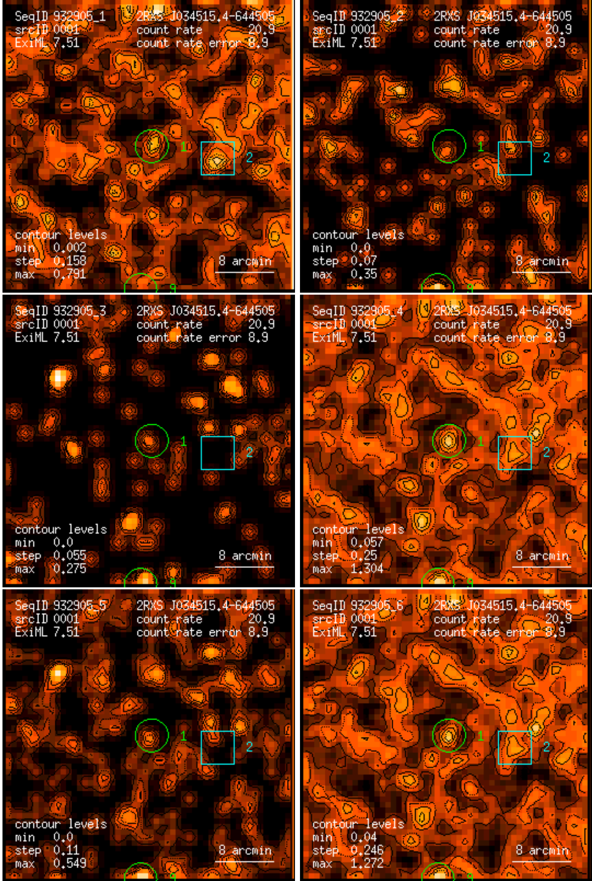
Figure 1: RASS 932905: detection 0001: band rate images, Gaussian filter: (1) PSPC channels 11 – 41, (2) 52 – 90, (3) 91 – 201, (4) 11 – 235, (5) 52 – 201, (6) 11 – 201. Broad band rates in counts/ks. Band rate contour levels in counts/ks/arcmin 2 .
