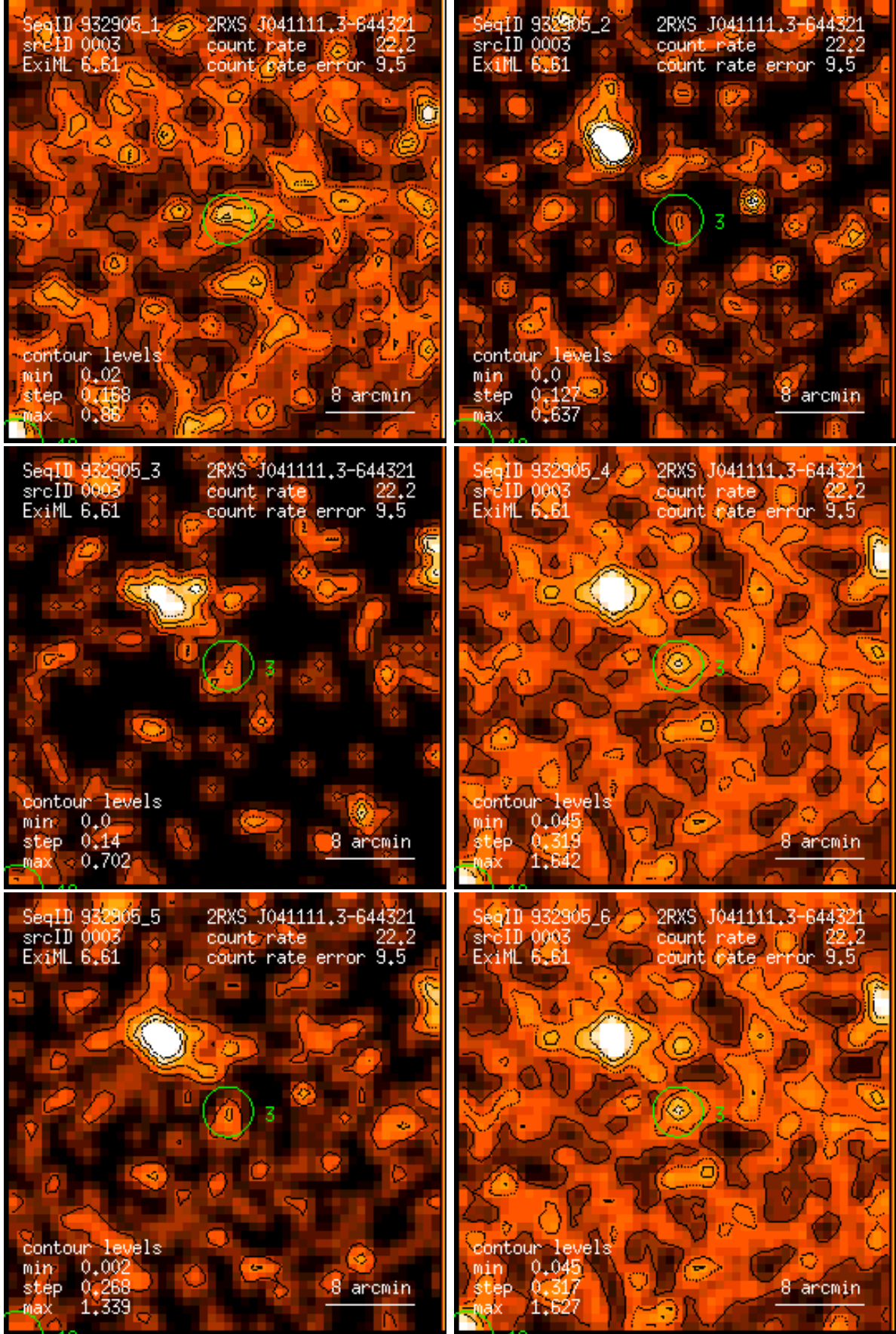
Figure 3: RASS 932905: detection 0003: band rate images, Gaussian filter: (1) PSPC channels 11 – 41, (2) 52 – 90, (3) 91 – 201, (4) 11 – 235, (5) 52 – 201, (6) 11 – 201. Broad band rates in counts/ks. Band rate contour levels in counts/ks/arcmin 2 .
