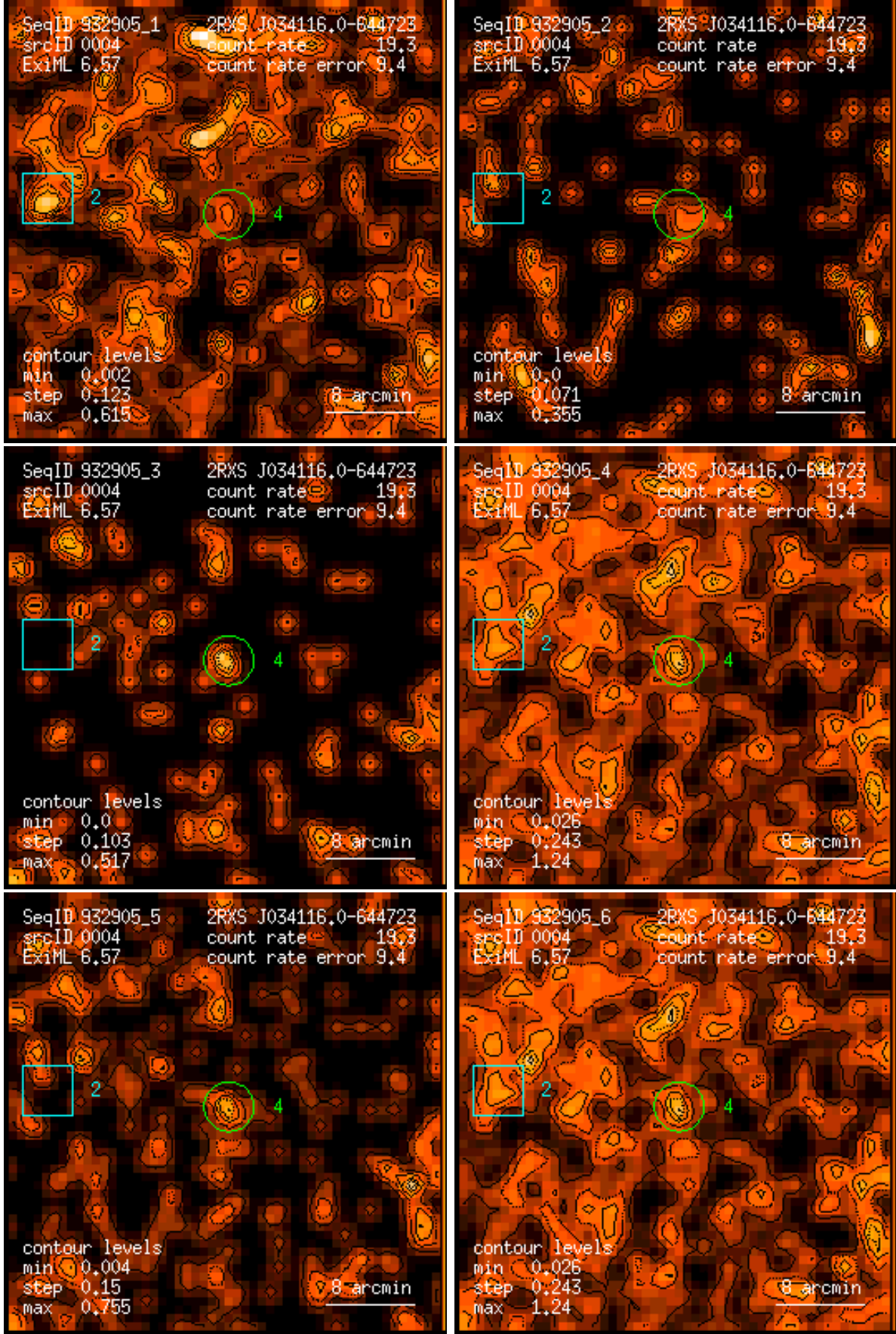
Figure 4: RASS 932905: detection 0004: band rate images, Gaussian filter: (1) PSPC channels 11 – 41, (2) 52 – 90, (3) 91 – 201, (4) 11 – 235, (5) 52 – 201, (6) 11 – 201. Broad band rates in counts/ks. Band rate contour levels in counts/ks/arcmin 2 .
