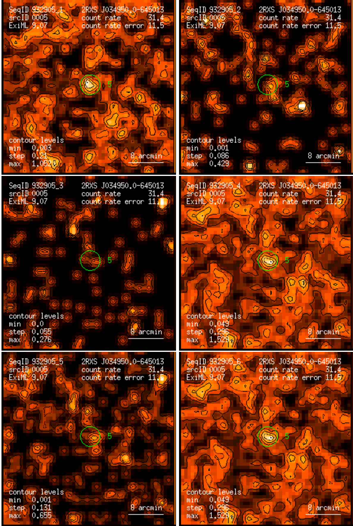
Figure 5: RASS 932905: detection 0005: band rate images, Gaussian filter: (1) PSPC channels 11 – 41, (2) 52 – 90, (3) 91 – 201, (4) 11 – 235, (5) 52 – 201, (6) 11 – 201. Broad band rates in counts/ks. Band rate contour levels in counts/ks/arcmin 2 .
