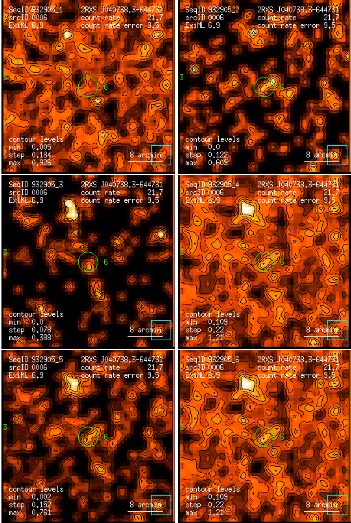
Figure 6: RASS 932905: detection 0006: band rate images, Gaussian filter: (1) PSPC channels 11 – 41, (2) 52 – 90, (3) 91 – 201, (4) 11 – 235, (5) 52 – 201, (6) 11 – 201. Broad band rates in counts/ks. Band rate contour levels in counts/ks/arcmin 2 .
